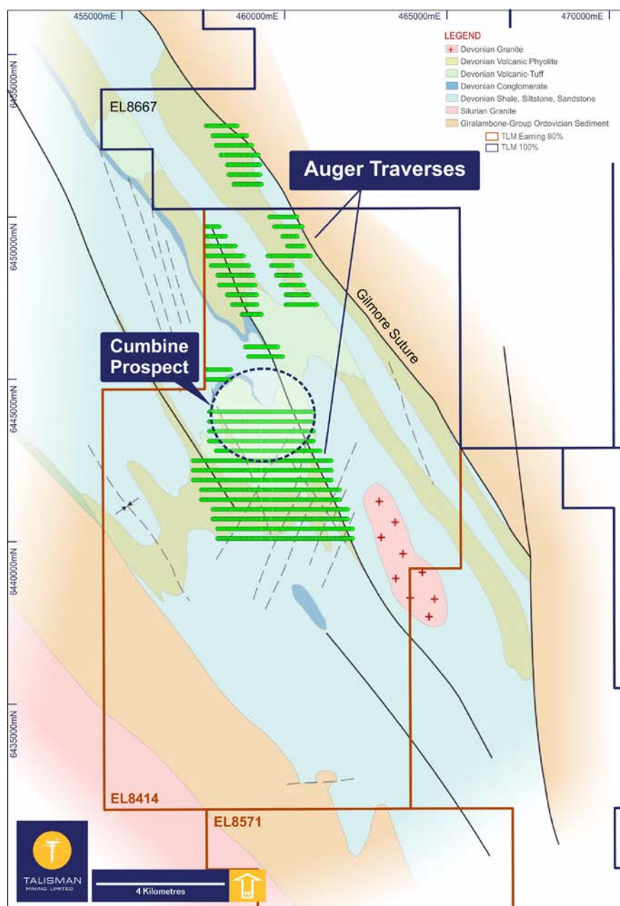
Figure 2: Phase 1 Auger drilling campaign – Bobadah Project area
