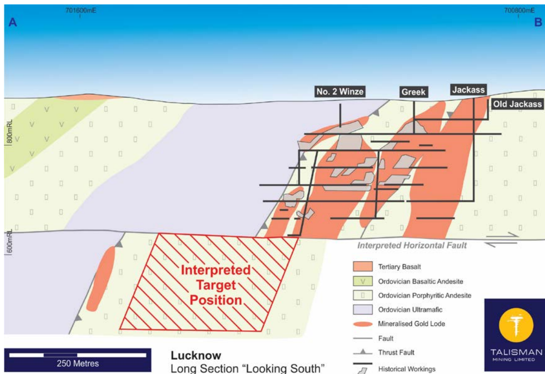
Figure 10: Lucknow Project interpreted long section, showing the interpreted faulted offset mineralisation target position.
