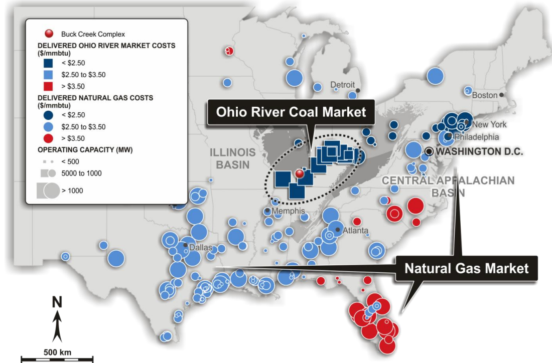
Figure 8: Ohio River Market Delivered Cost of Coal ($/mmbtu) vs. Regional Delivered Cost of Natural Gas ($/mmbtu)
