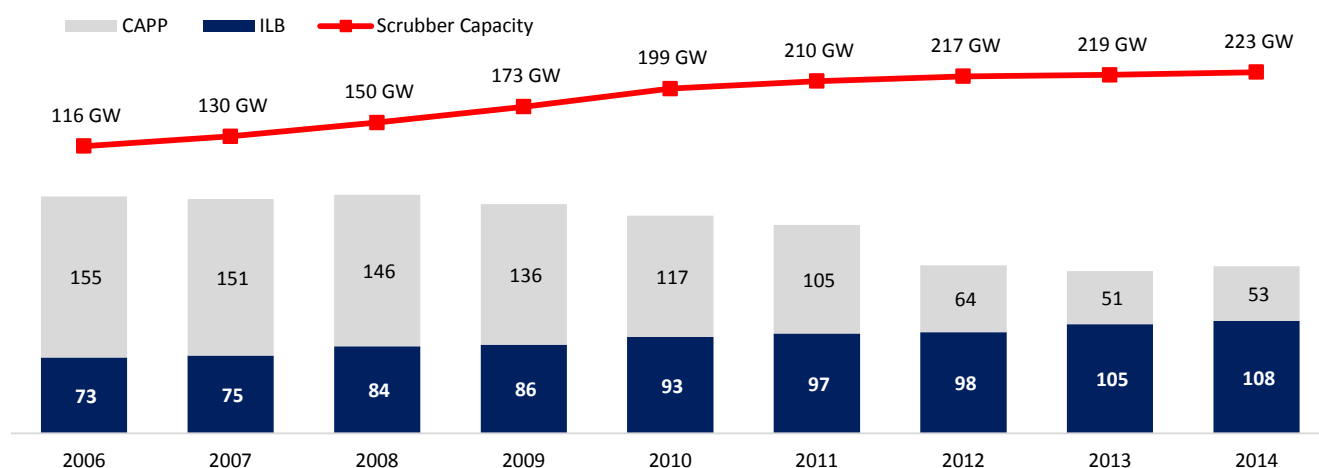
Figure 5: ILB and CAPP Coal Deliveries compared with US Scrubber Capacity Additions
