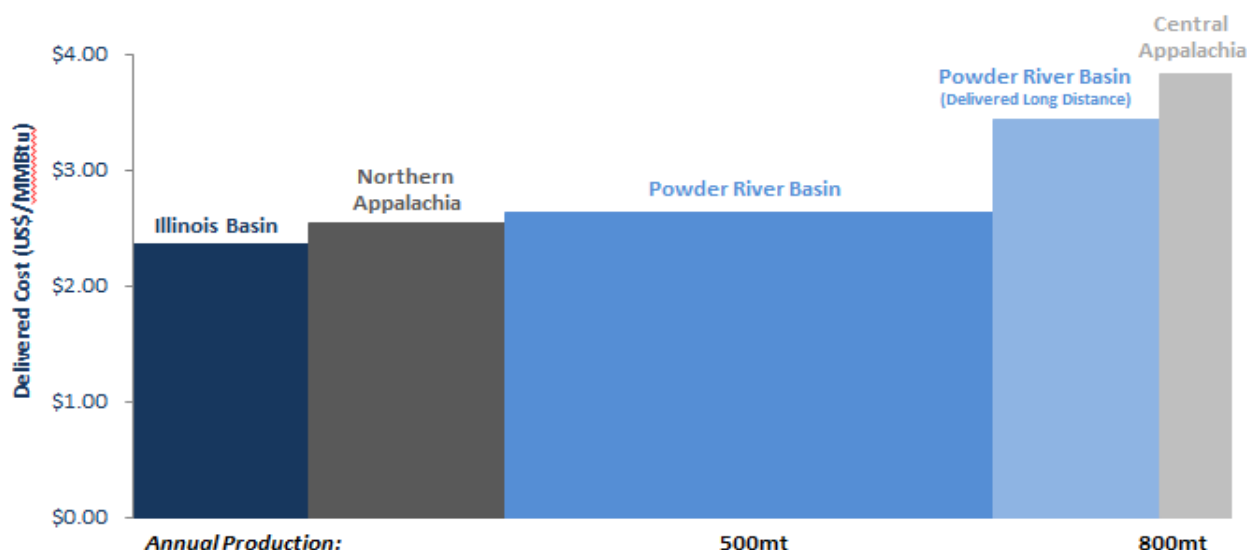
Figure 4: Major US Coal Basin Delivered Cost Curve to Eastern US Power Markets
