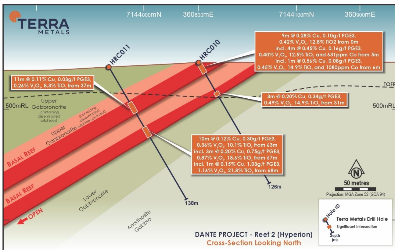
Figure 6. Cross Section HRC011-HRC010 from the Hyperion Reef.
