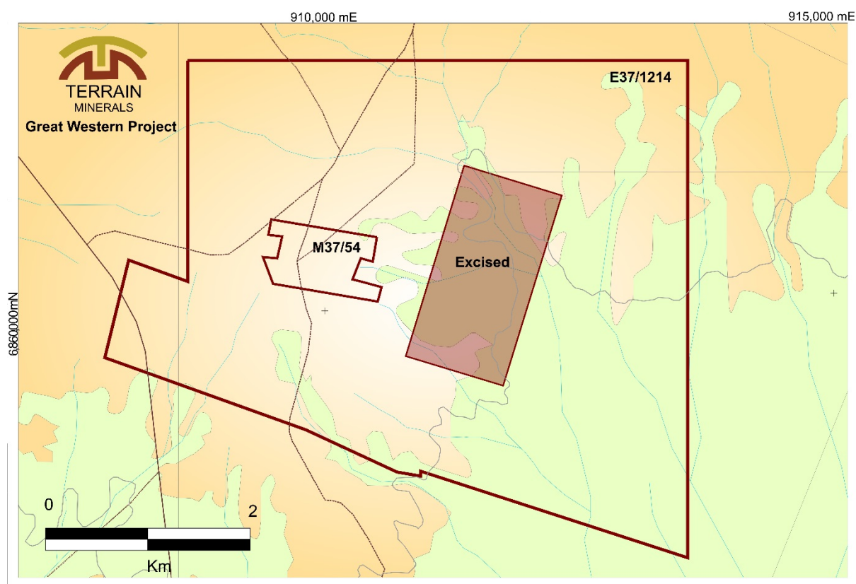
Figure 4: E37 / 1214 surrounding area around the Great Western Project M37 / 54
