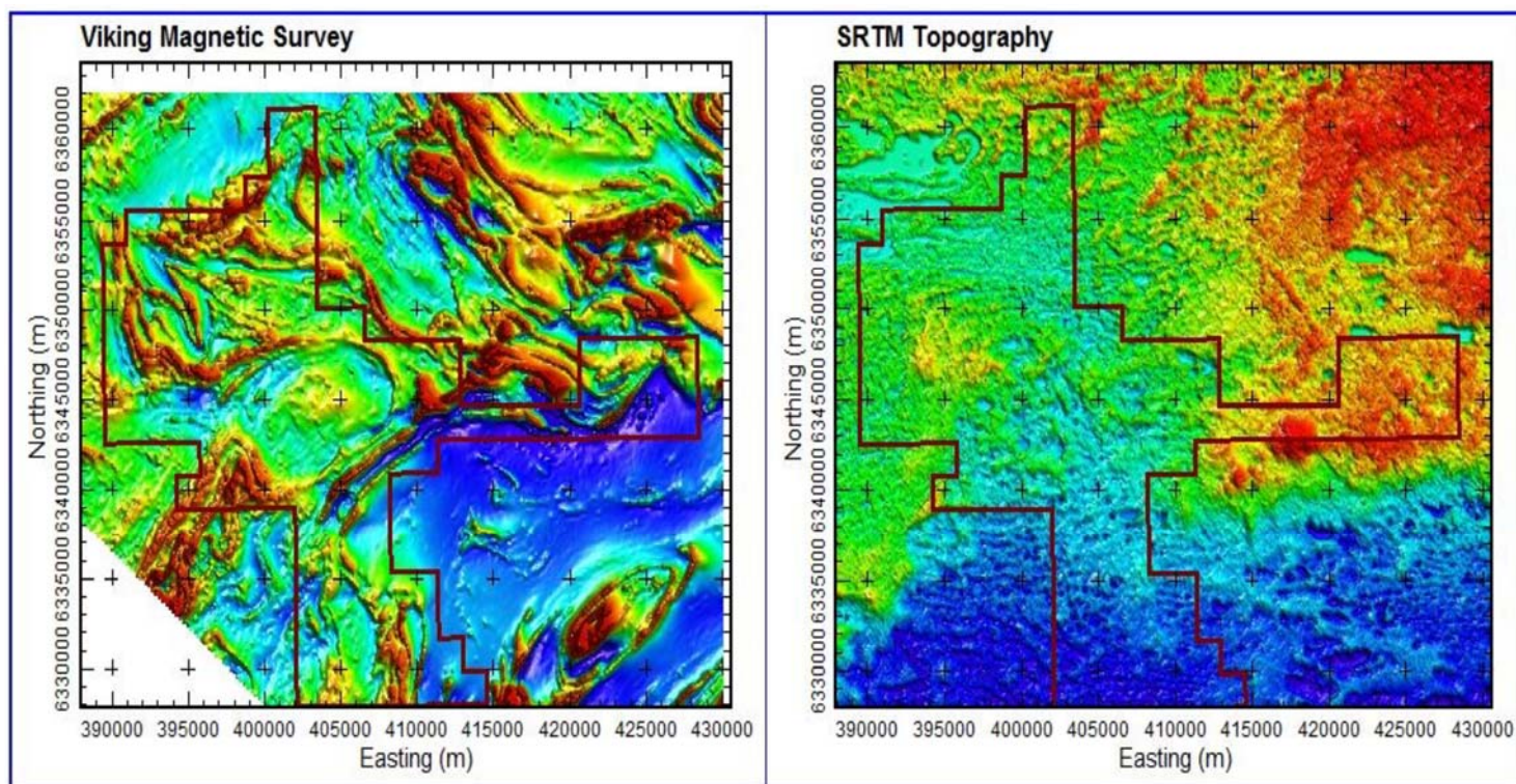
Figure 5: Overview of project area and E63_1740_TMX; magnetics (left) and topography (right)
