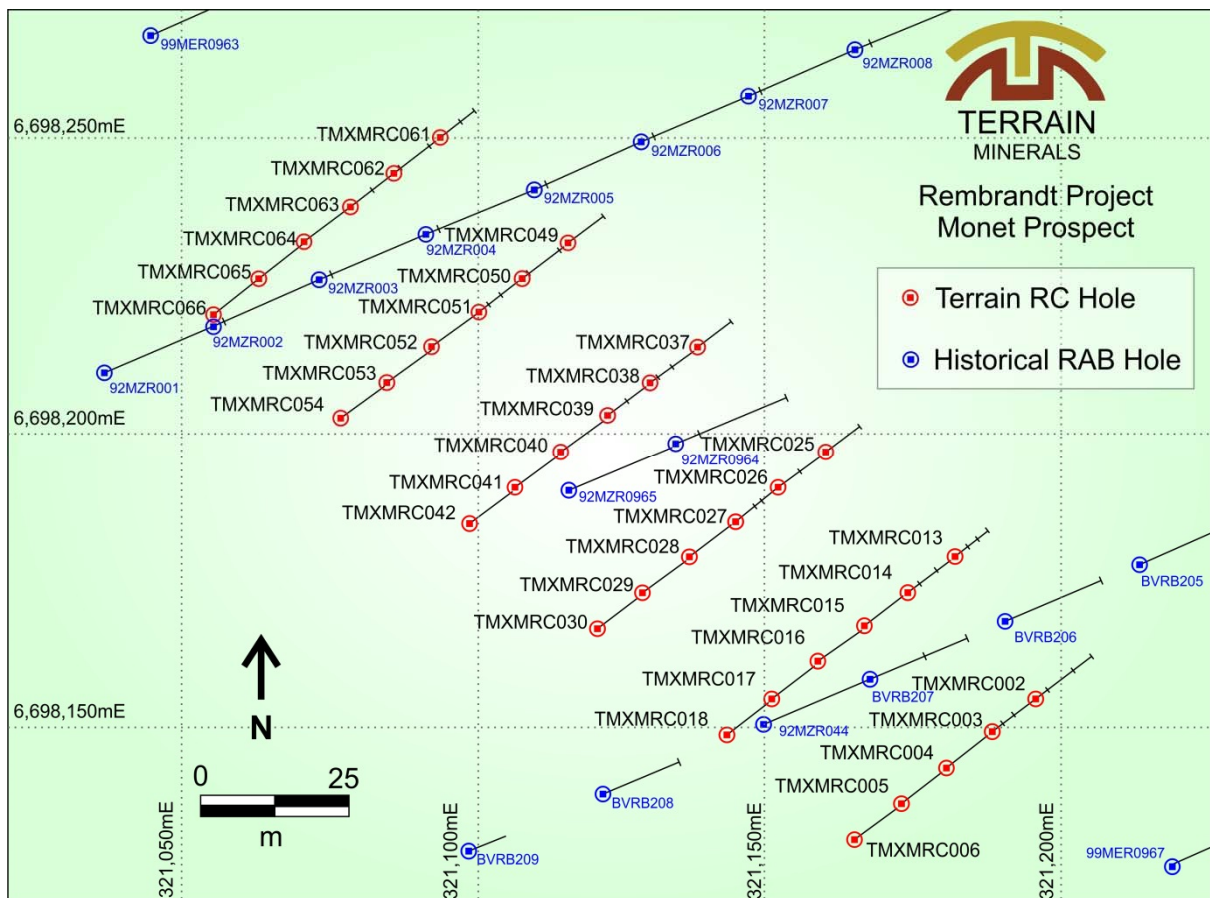
Figure 3: Monet Prospect Drill Collar Plan
