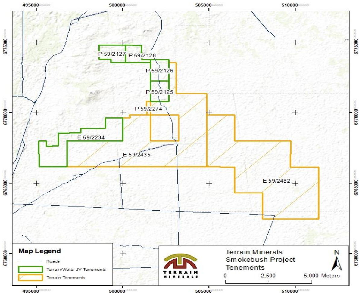
Diagram 5: Smokebush Project Location (tenements 100%). The new Hurley IP target is located on P59/2126 with the other target located on P59/2125 and north of Paradise city which is located on E59/2435. Monza is located on P59/2128.
