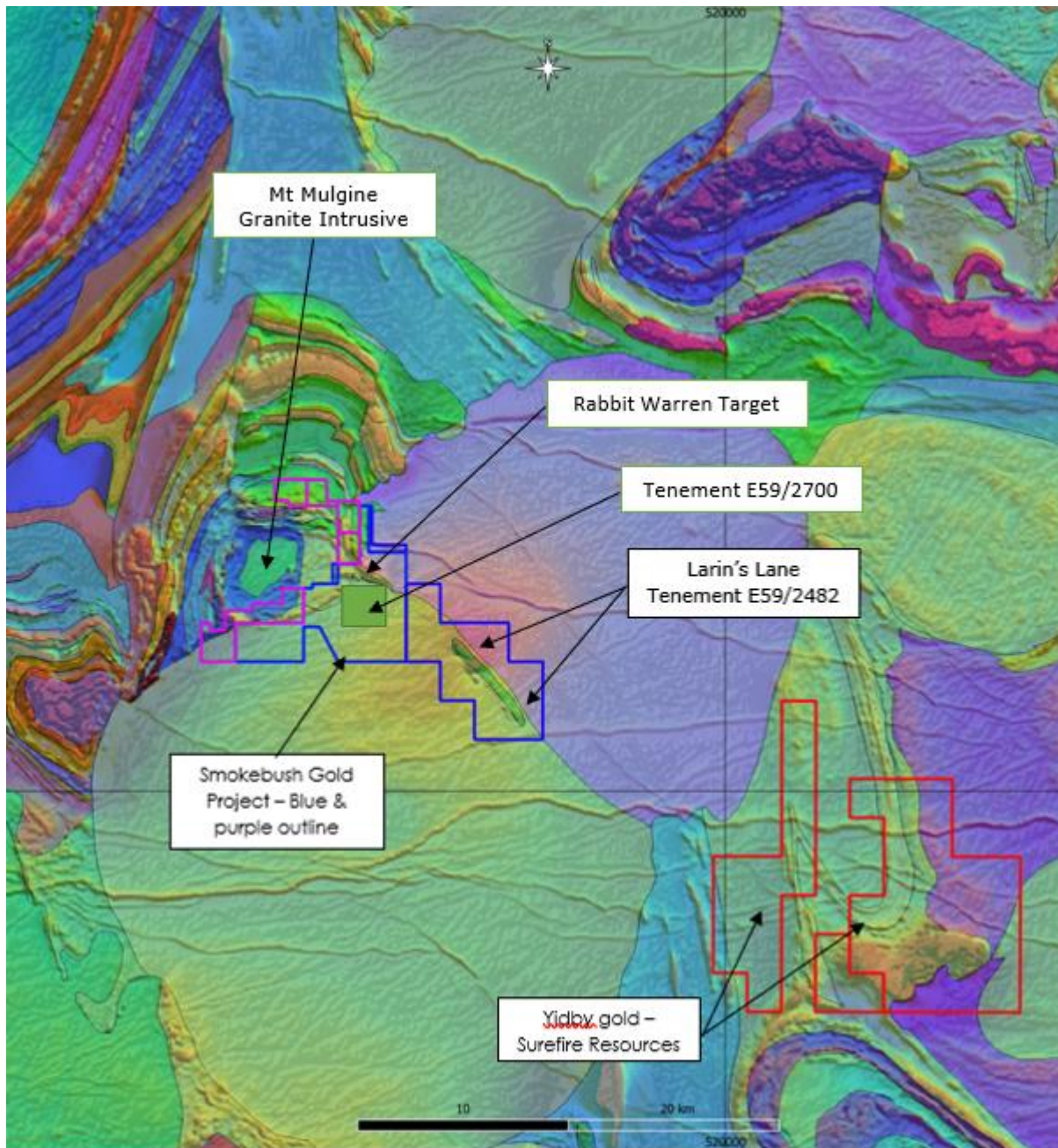
Diagram 4: Smokebush Project Location: The Mt Mulgine granite intrusive can be identified and shows that Terrain pegmatites are in the so-called Goldilocks zone for potential lithium mineralisation. The area also hosts Terrains new Larin's Lane gold target a ~4.5km long by 200-300m wide untested and undercover greenstone that is wedged between two granites.
