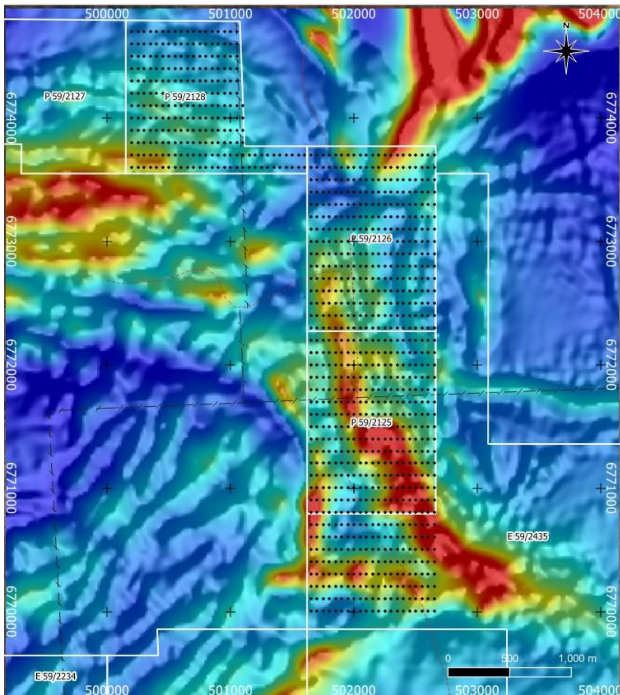
Diagram 3: The above plan shows the survey points for the current Induced Polarisation (IP) survey. The specifications and details of the IP survey include 200 metre line spacing (with infill 100 metre line spacing order any anomaly), and 50 metre along line sample spacing.
