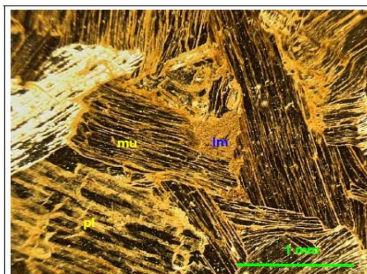
Sample 11 Platy muscovite (mu) with limonite flooding along cleavages occurring in the weathering profile. Limonite (lm) occurs interstitially and may have replaced original sulphides (arrowed). Plane polarised incident light. Crossed polars. Field of view – 3.7 mm.
