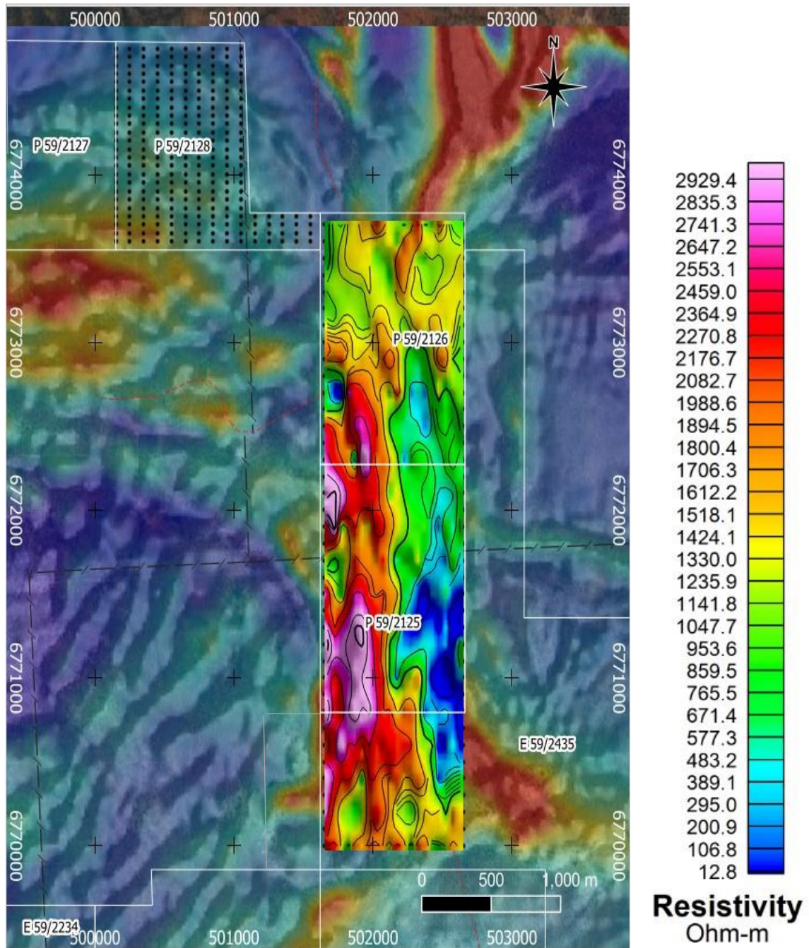
Diagram 2. Smokebush Gradient Array IP Chargeability with Contours
