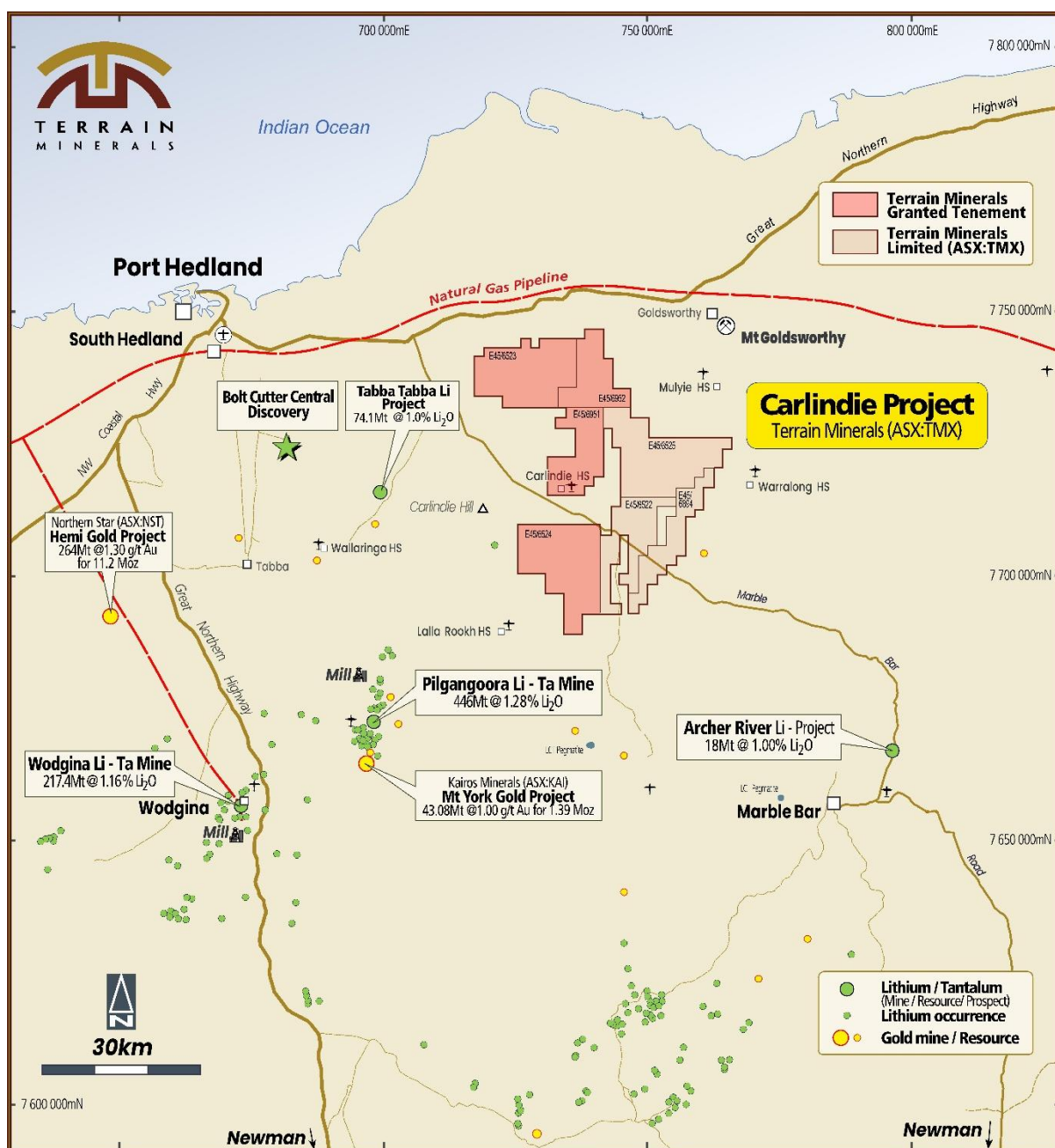
Diagram 1. Location of the Carlinde Project within the East Pilbara, approximately 90 kilometres southeast of Port Hedland, Western Australia. The Project is strategically positioned between Wildcat Resources' (ASX: WC8) Tabba Tabba lithium deposit and SQM-Kali Metals' (ASX: KM1) Pilbara lithium ground in a province that also hosts Pilbara Minerals' Pilgangoora operation and Mineral Resources' Wodgina lithium mine.
