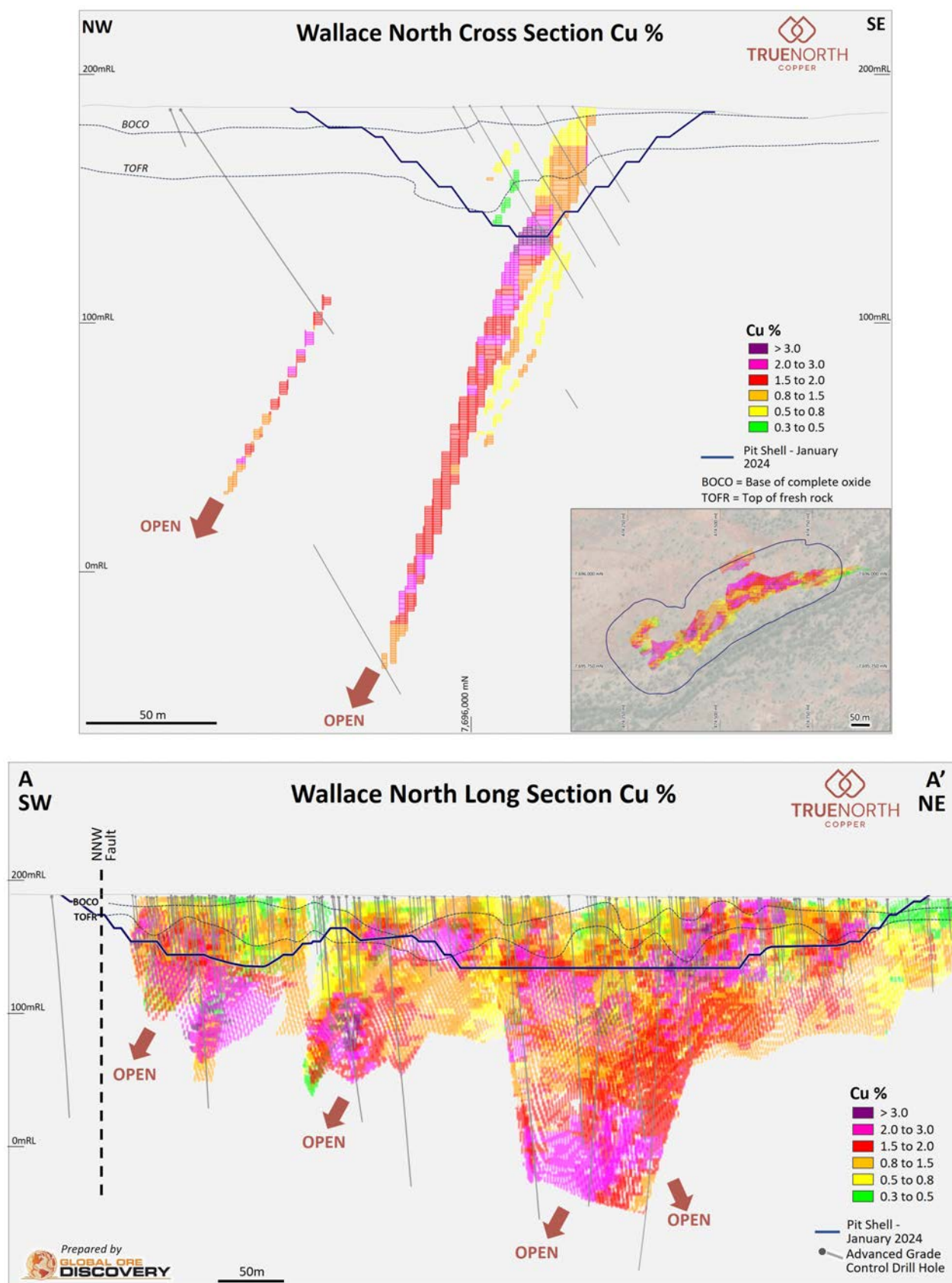
Figure 3. Wallace North Project mineral resource block model cross section (top) and long section with MEC designed Pit outline 3,4 . Oxide (BOCO) and sulphide (TOFR) ore boundaries also shown.
