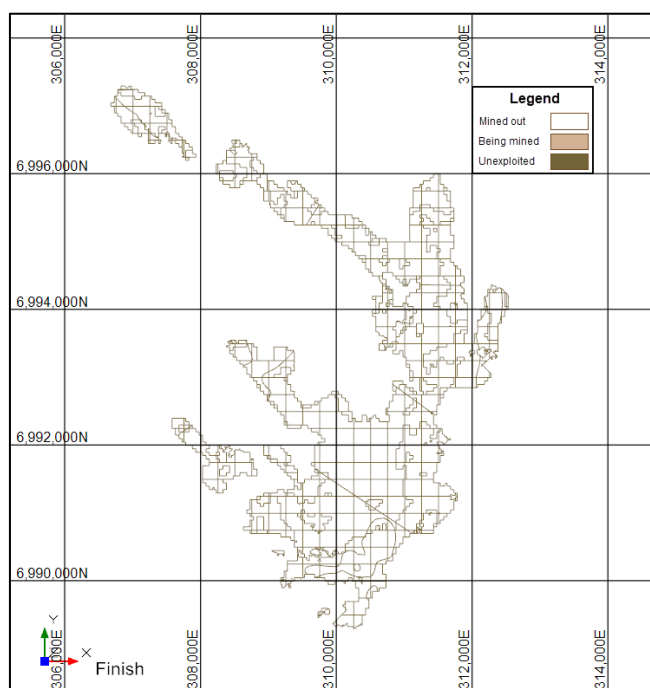
Figure 22: Projected pit at end of Year 20
