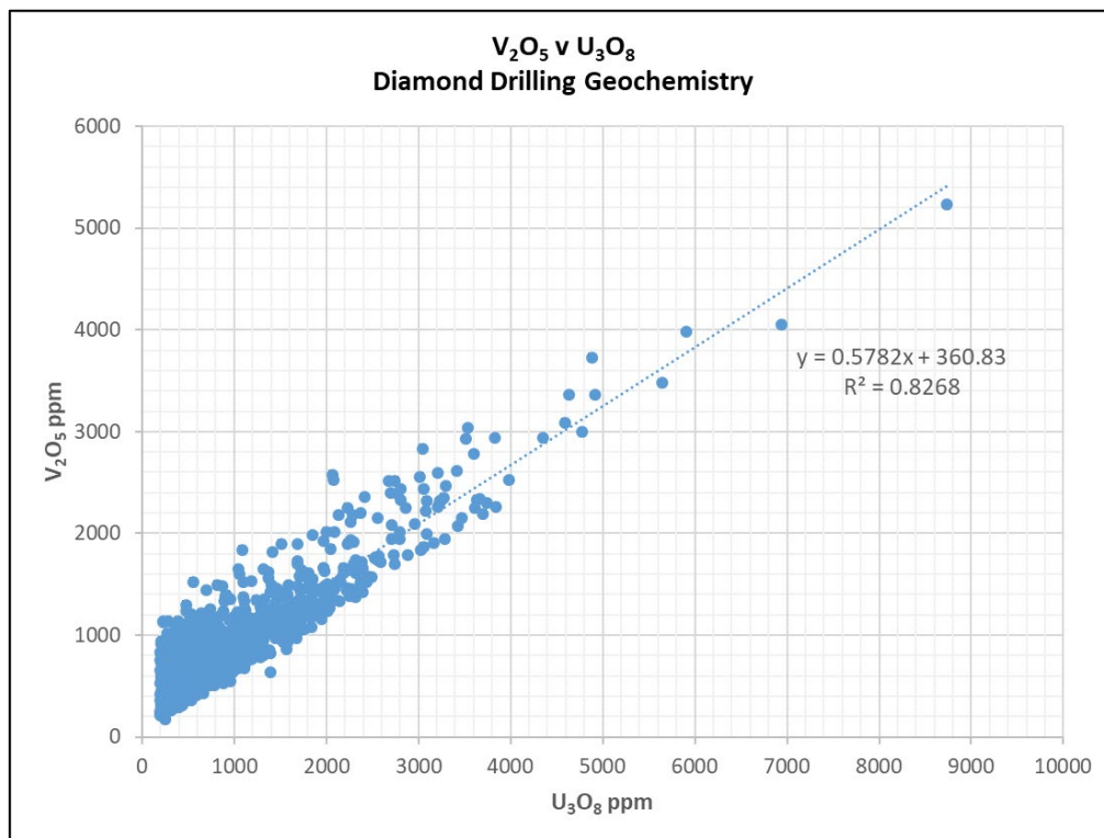
Figure 9: Bivariate plot showing the relationship between U_3O_8 and V_2O_5 (calculated from U and V respectively) in the geochemistry from all diamond holes inside the 200ppm U_3O_8 cut-off within the Lake Maitland U_3O_8 resource.
