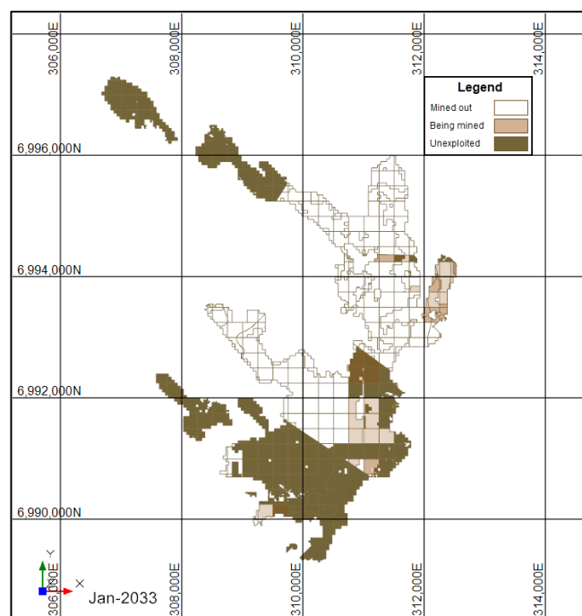
Figure 20: Projected pit at end of Year 10
