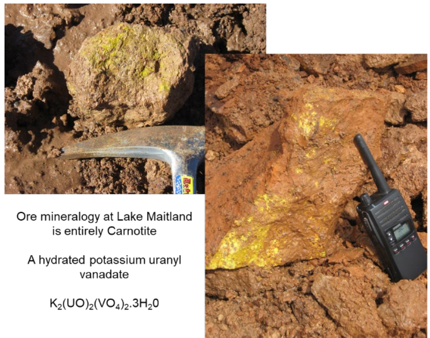
Figure 5: Photographs of the yellow 'ore' mineral, carnotite, of Toro's shallow groundwater carbonate related uranium deposits, inclusive at Lake Maitland.
