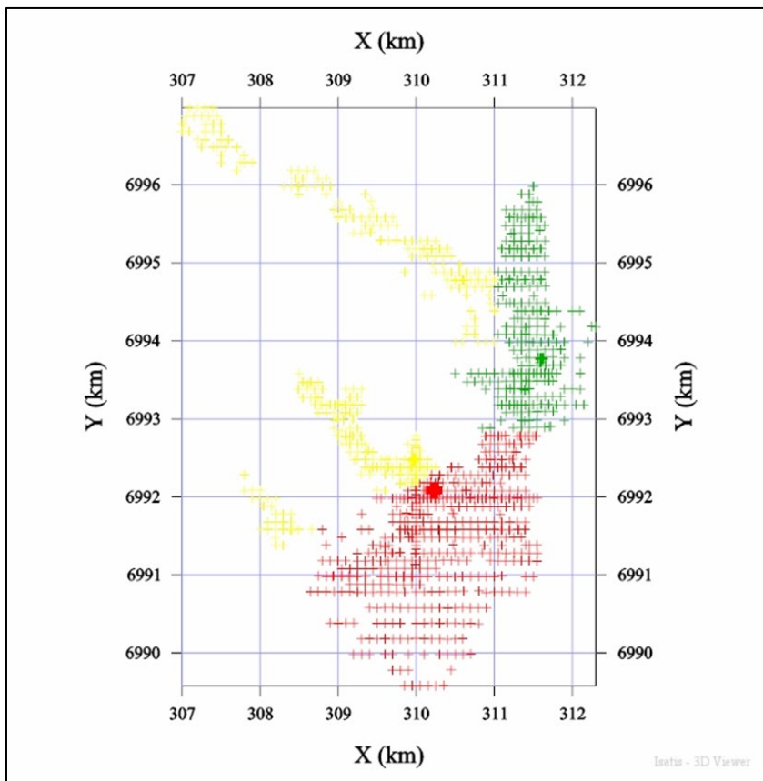
Figure 8: Lake Maitland Domaining (D1 green, D2 red and D3 yellow)
