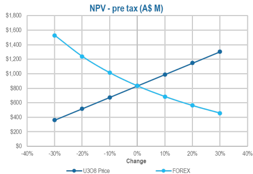
Figure 2: Lake Maitland Project Uranium Price Sensitivities Uranium Price (US$/lb U3O8) – (A$:US$ 0.70)
