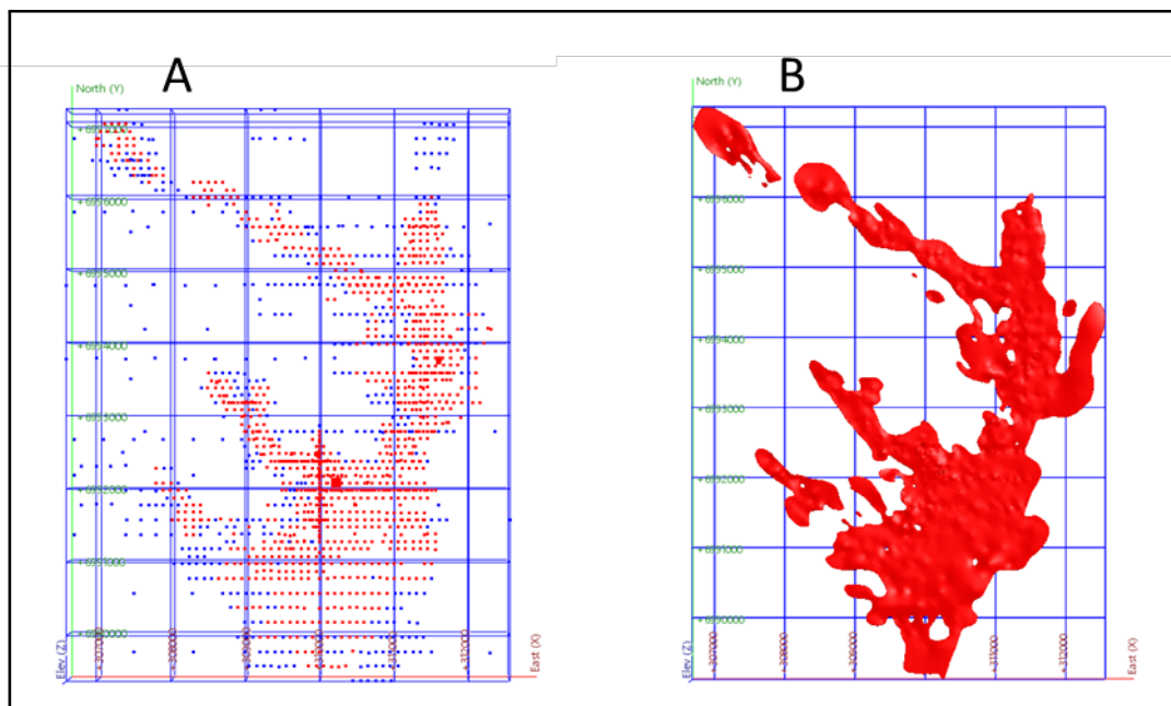
Figure 7: (A) Indicator data, in red all holes with a maximum 0.5m composite value over 1000ppm (included) and in blue all holes without a maximum 0.5m composite value of 100ppm (discarded). (B) Final Lake Maitland 100 ppm mineralisation envelope in plan view.
