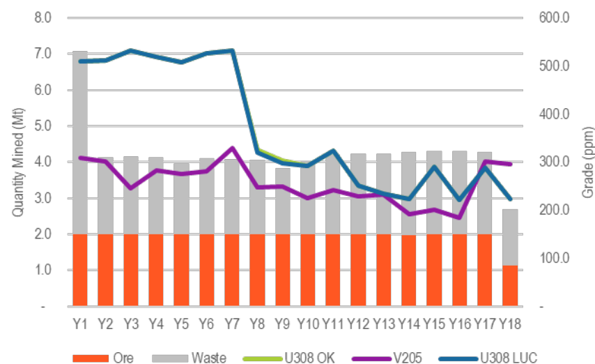
Figure 11: LoM mining production schedule – diluted tonnes and grades mined.
