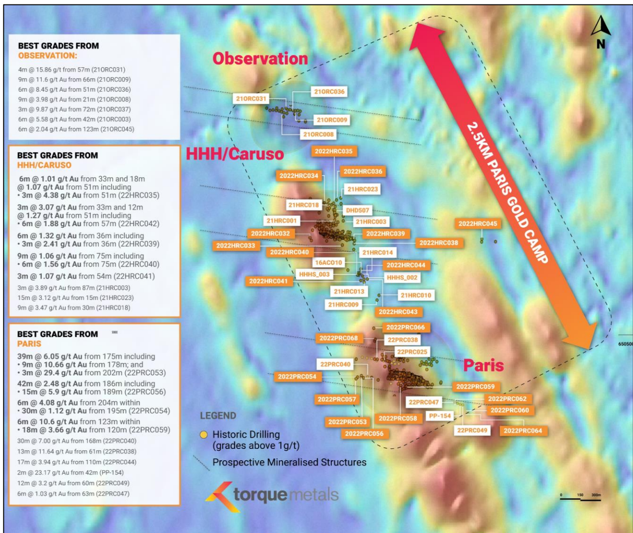
Figure 4: Paris Gold Camp
