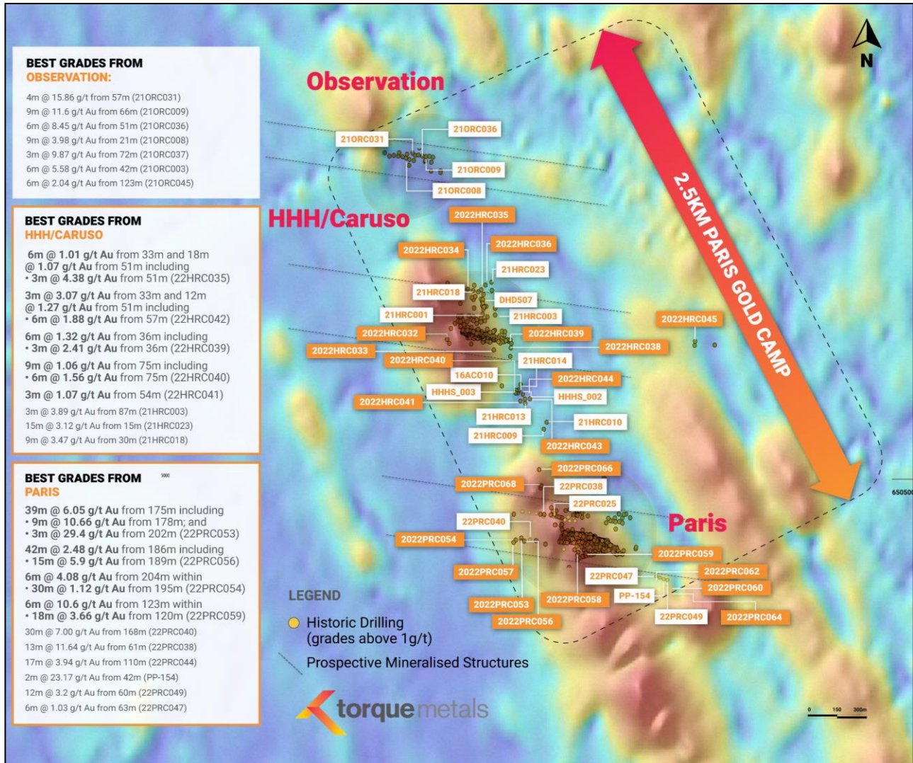
Figure 6: Paris Gold Camp
