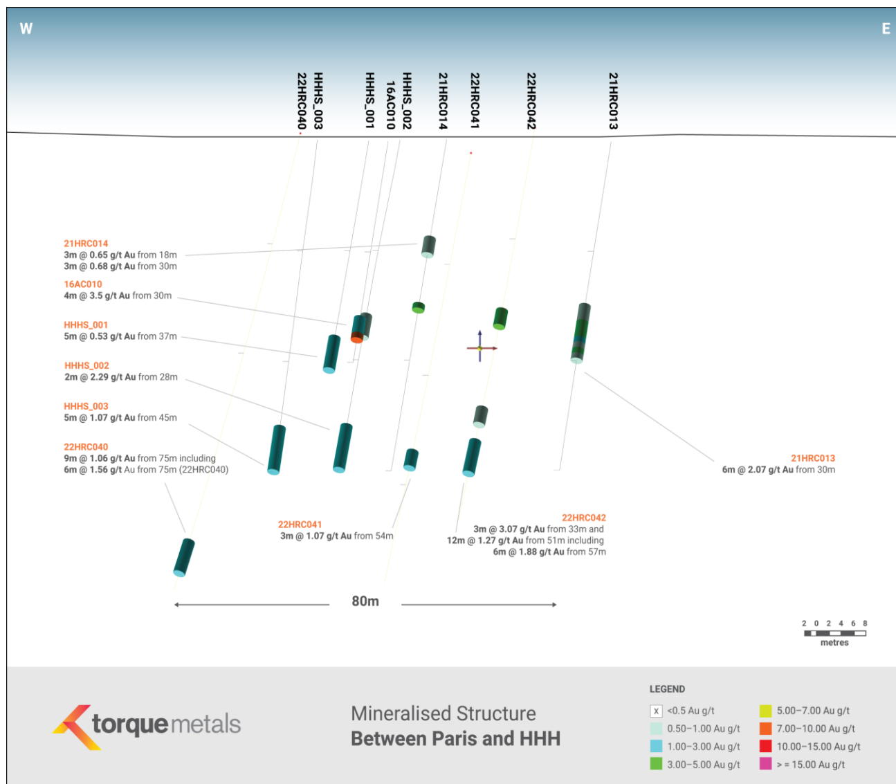
Figure 3: Cross-section of holes between Paris and HHH 5,6
