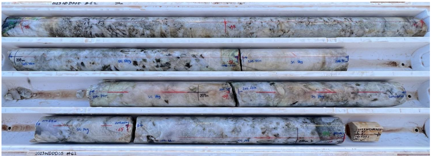
Figure 3 Diamond core 23NDD005 from 207.06m to 210.10m from New Dawn Lithium Project. Note that assays for this hole were received.
