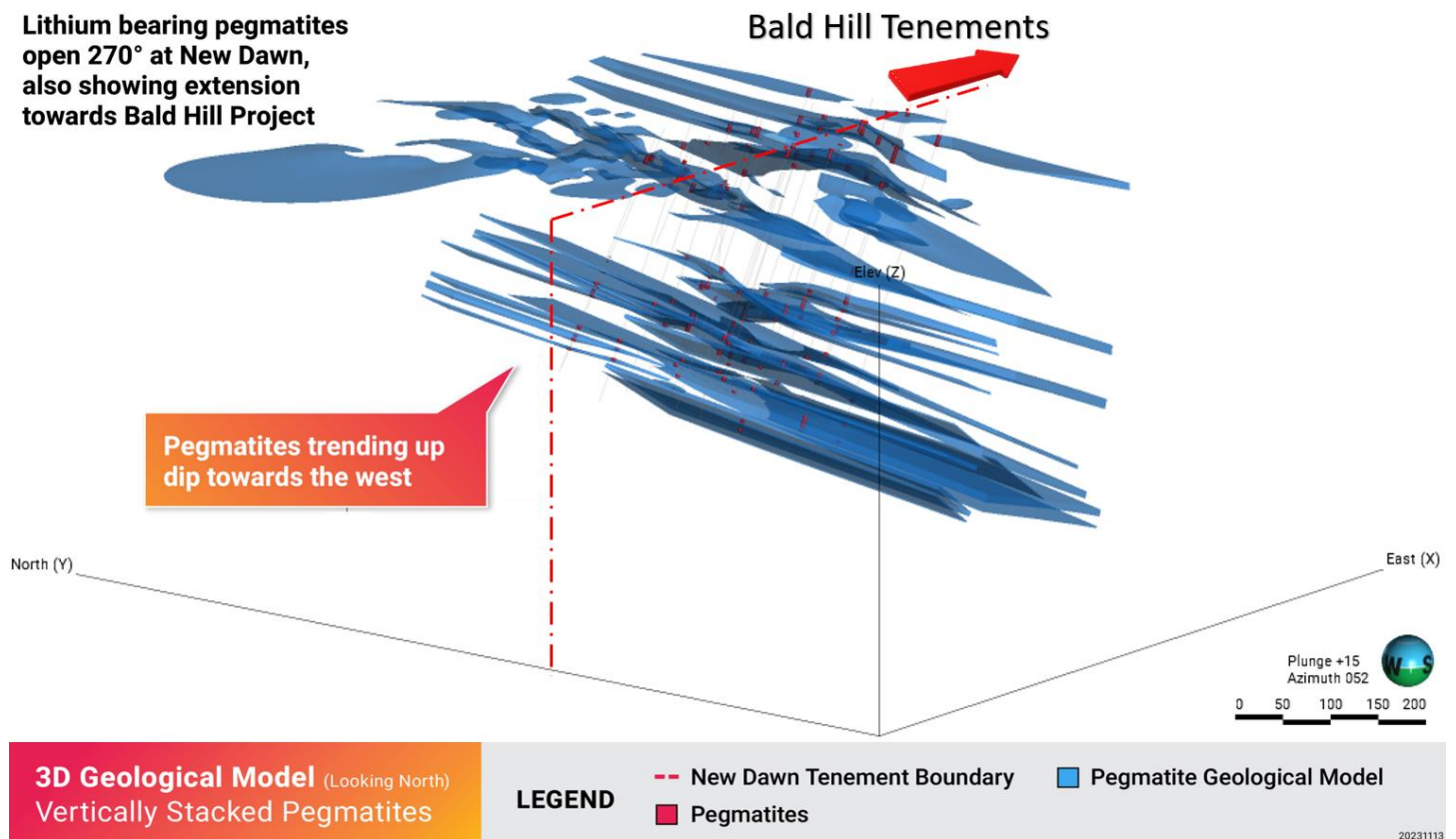
Figure 11 3D Geological model showing vertically stacked pegmatites open 270 degrees.
