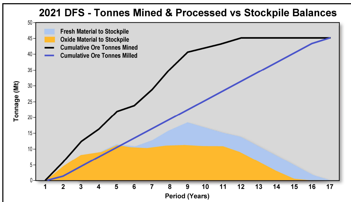
Figure 1: Cumulative Ore Mined and Processed with Annual Stockpile Balances for the Kobada Project (source: 2021 DFS)
