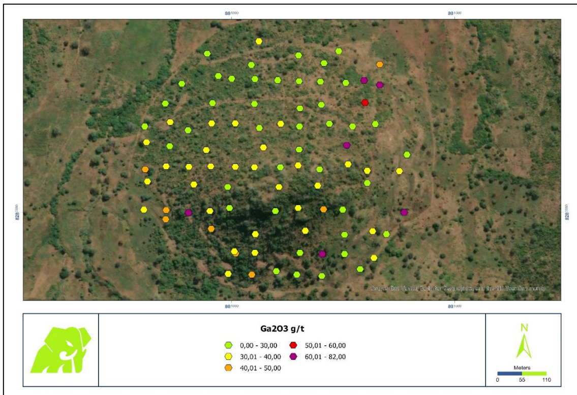
Figure 4: Map showing the surface distribution of wide-spread Gallium mineralisation at Nathace Hill, Tundulu Project.
