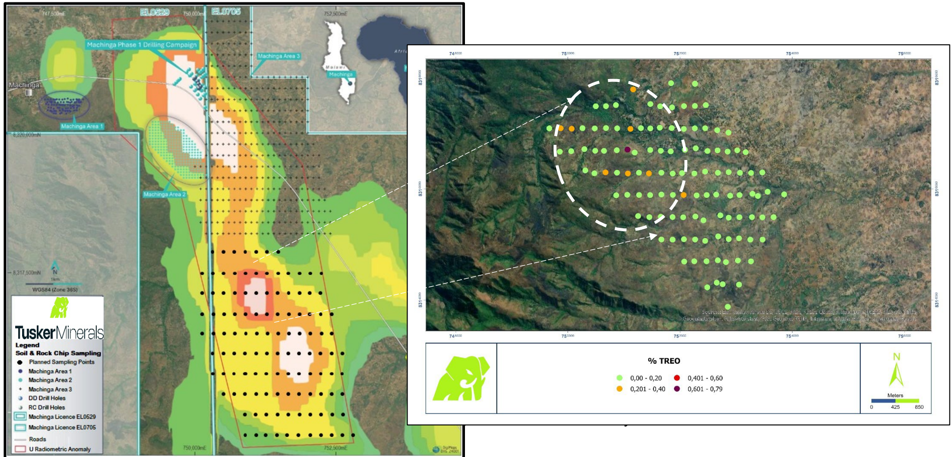
Figure 7: Map of the Machinga Project showing planned & sampled locations across the large U radiometric anomaly that has returned up to 0.79% TREO.
