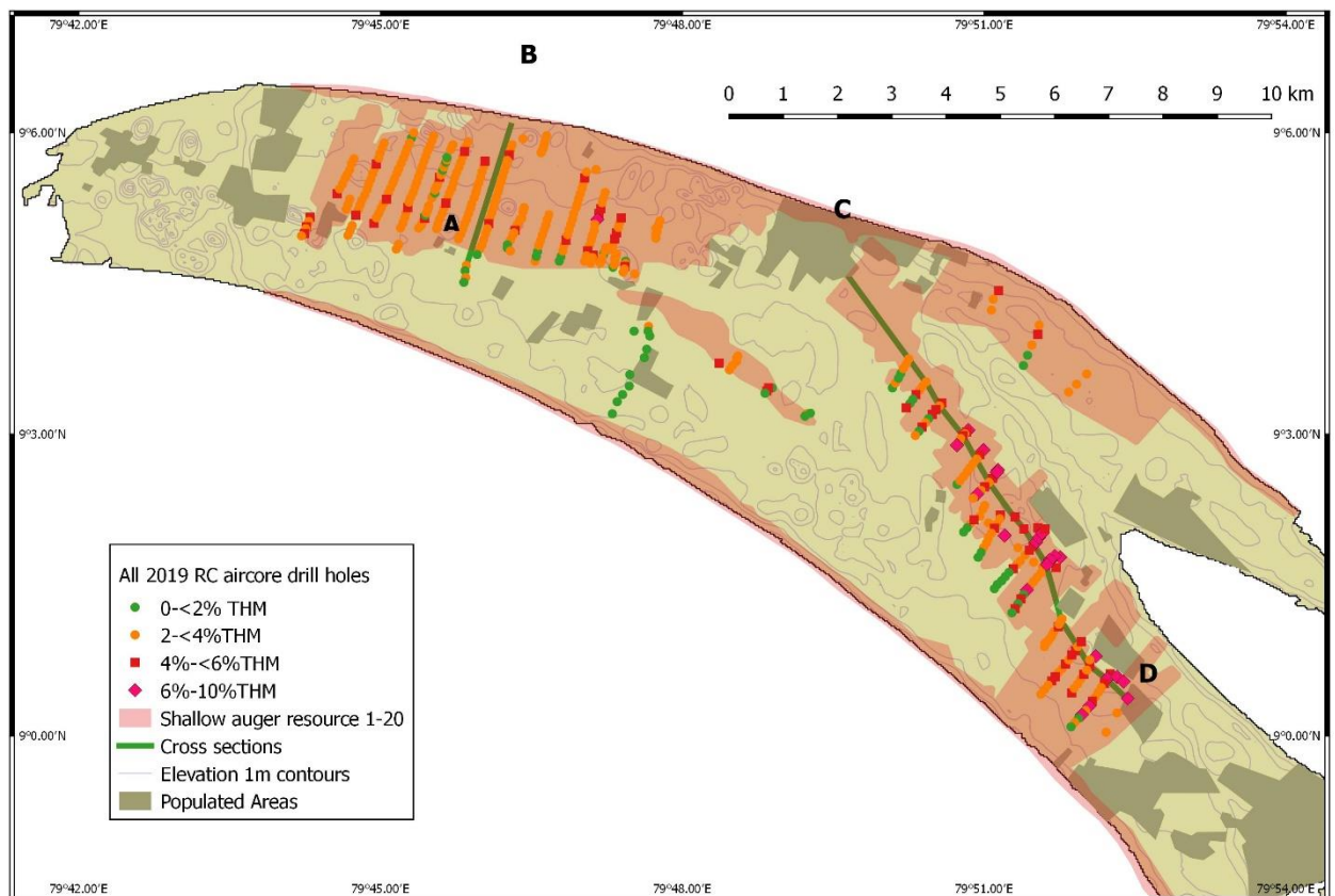
Figure 1 Location of the RC aircore drill holes and sections in Figures 2 and 3.
