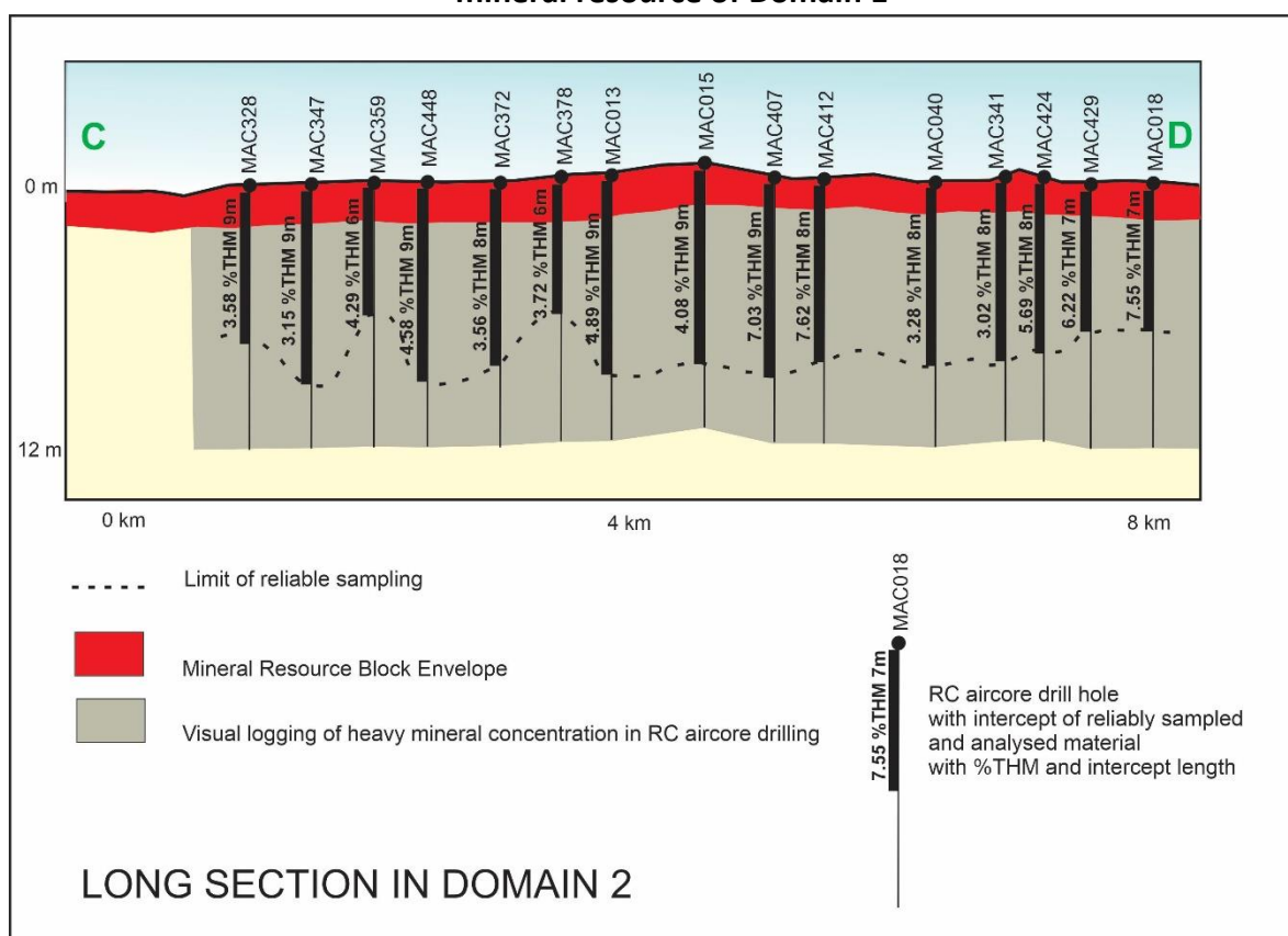
Figure 3 Long section C-D (located on Figure 1) showing RC drilling results beneath existing mineral resource of Domain 2
