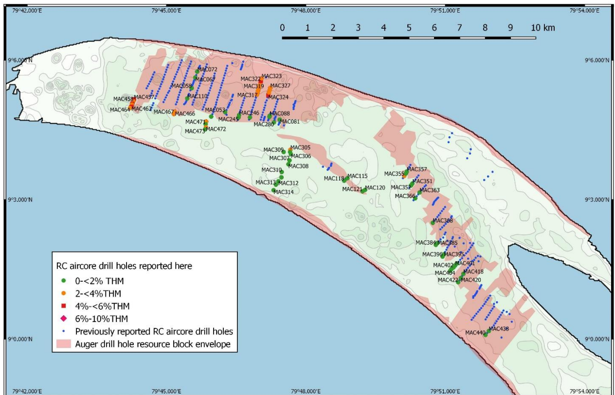
Appendix Figure 1 Location all previously reported RC aircore drill holes (blue) and the 76 new drill holes reported here ( colour coded and numbered).
