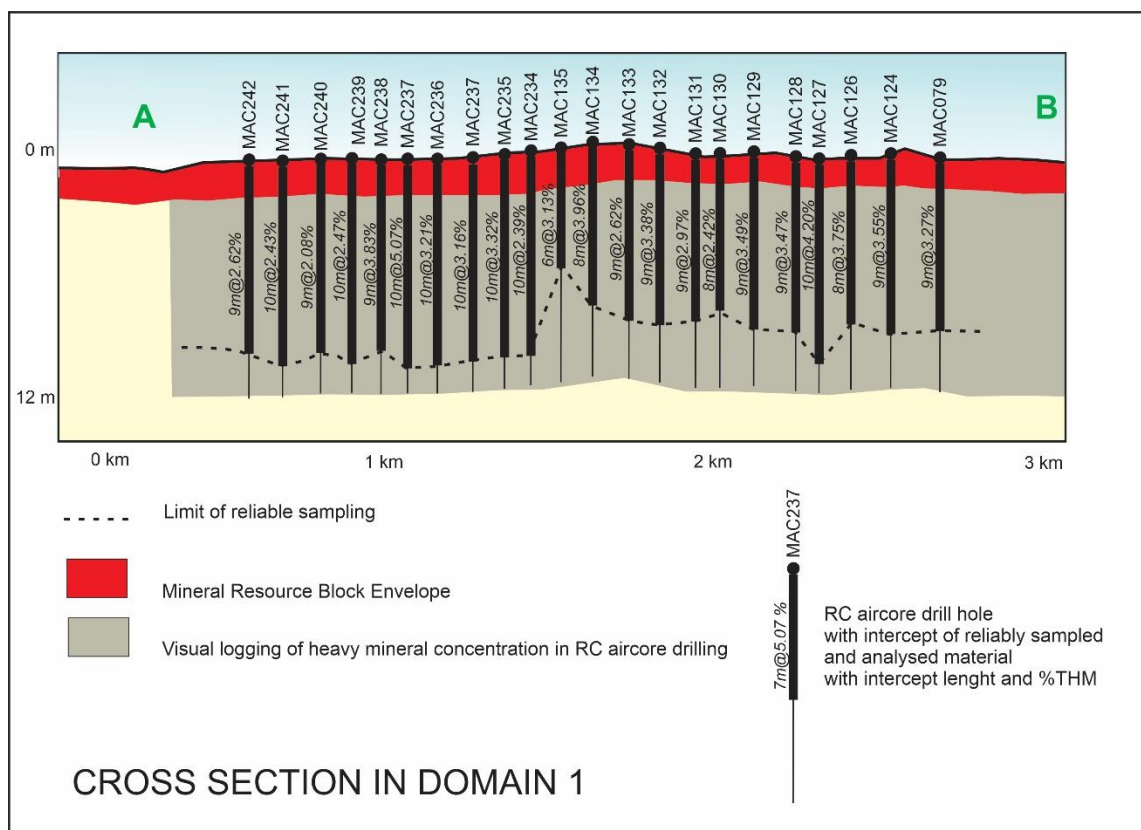
Figure 2 Cross section A-B (located on Figure 1) showing RC drilling results beneath existing mineral resource of Domain 1
