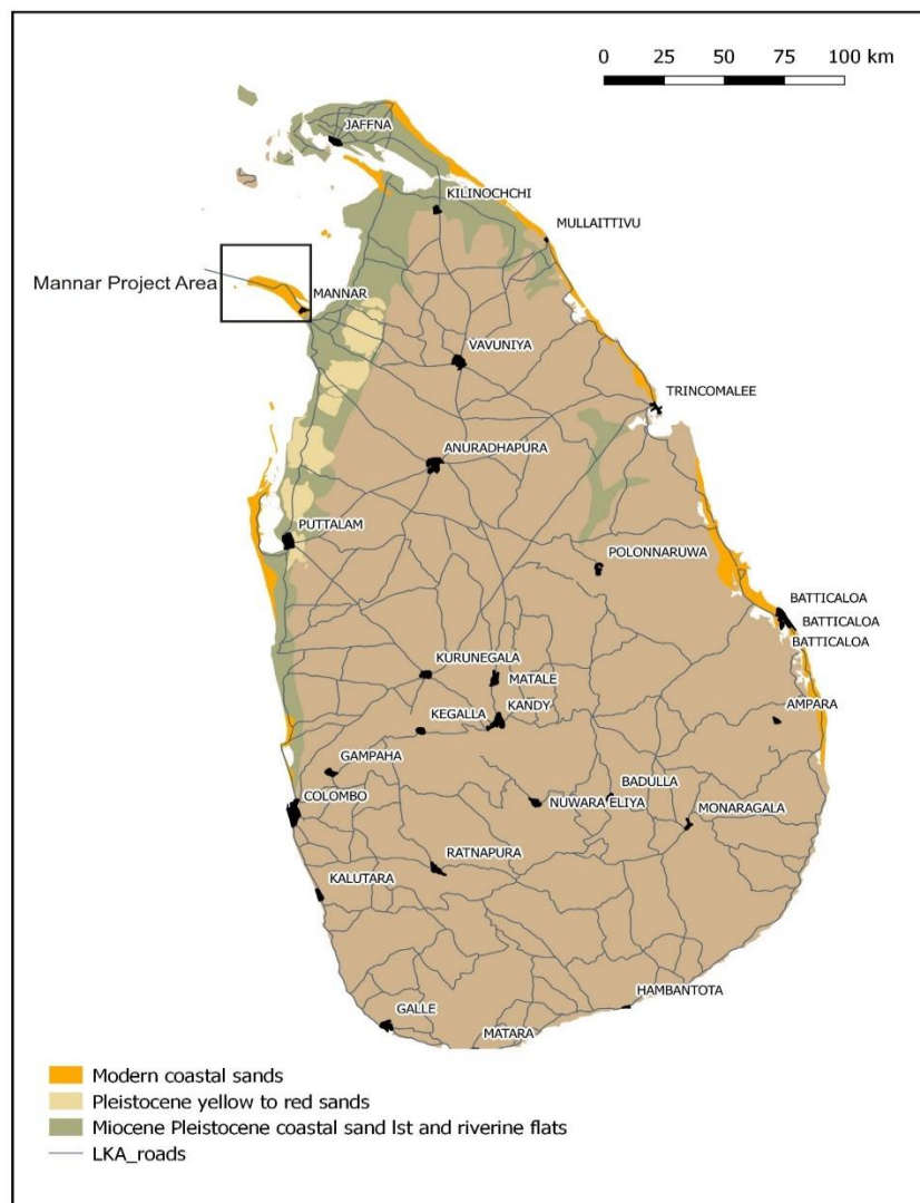
Figure 5 Location of the Mannar island Project in NW Sri Lanka
