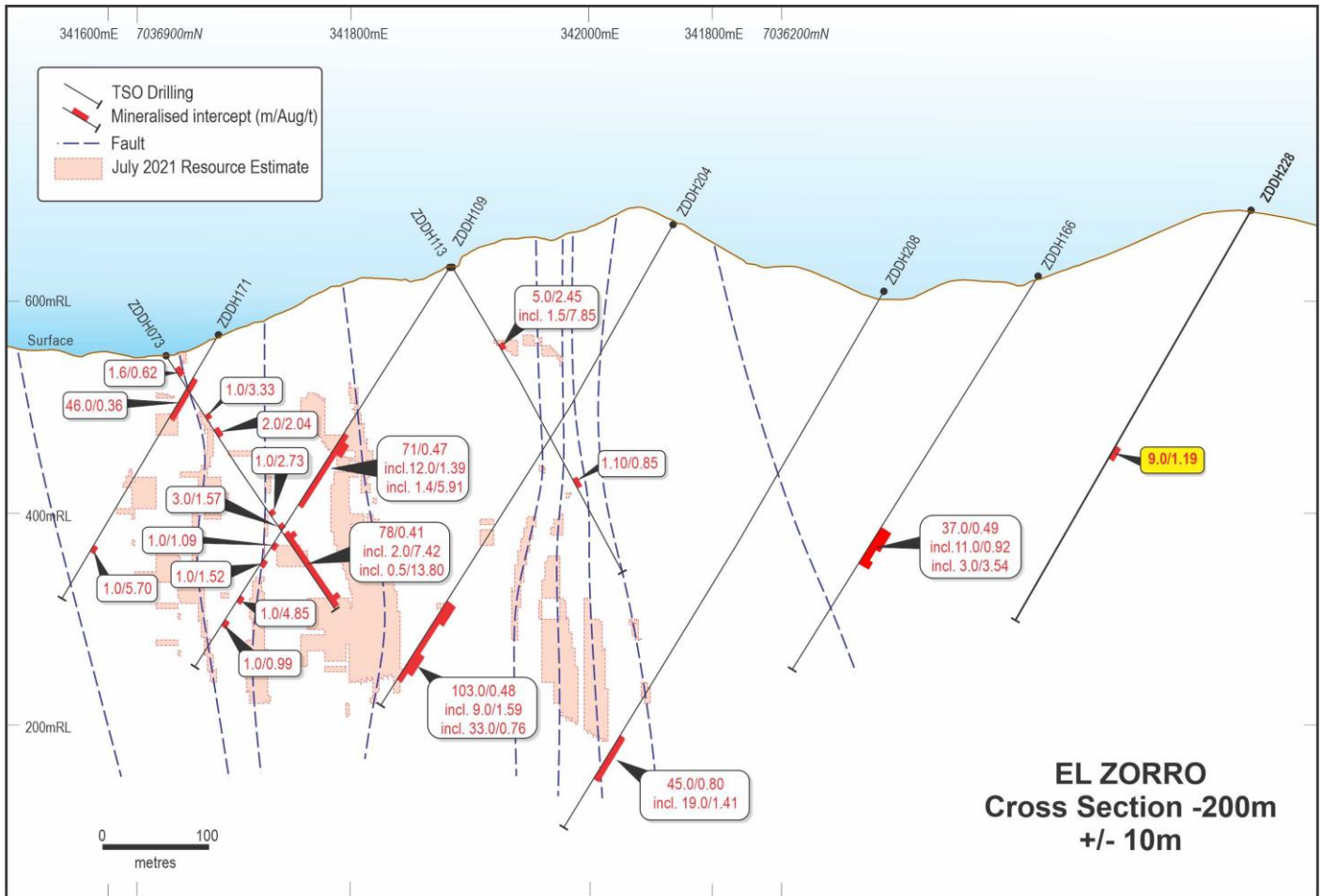
Figure 4: Terner Drill Section -200m, hole ZDDH0228 intersected new gold zone at Terner East.
