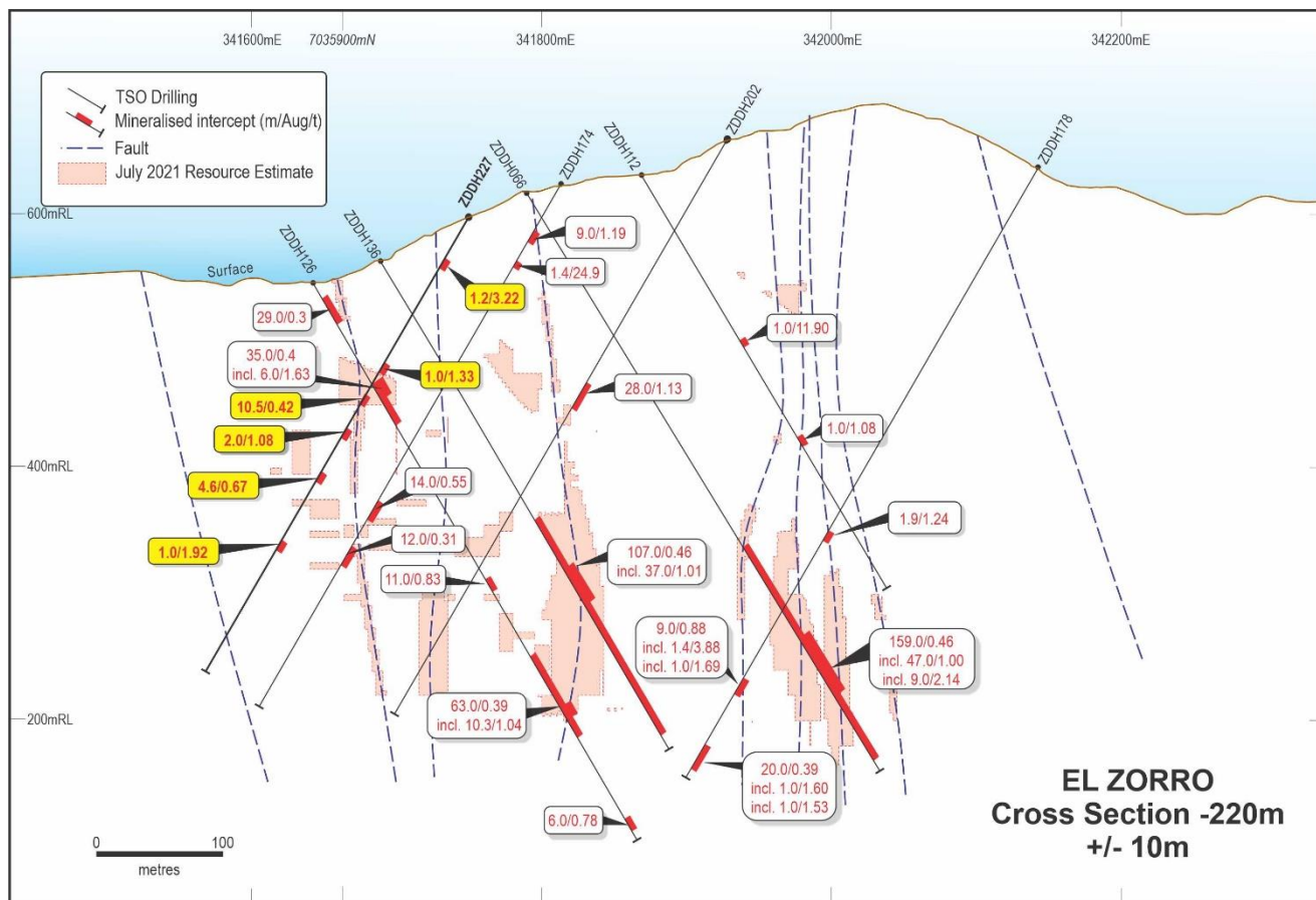
Figure 5: Terner Drill Section -220m looking northwest.
