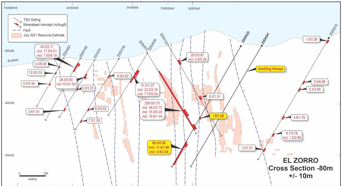
Figure 2: Terner Drill Section -80m looking northwest. Hole ZDDH0225 extending depth of mineralisation by >100m.
