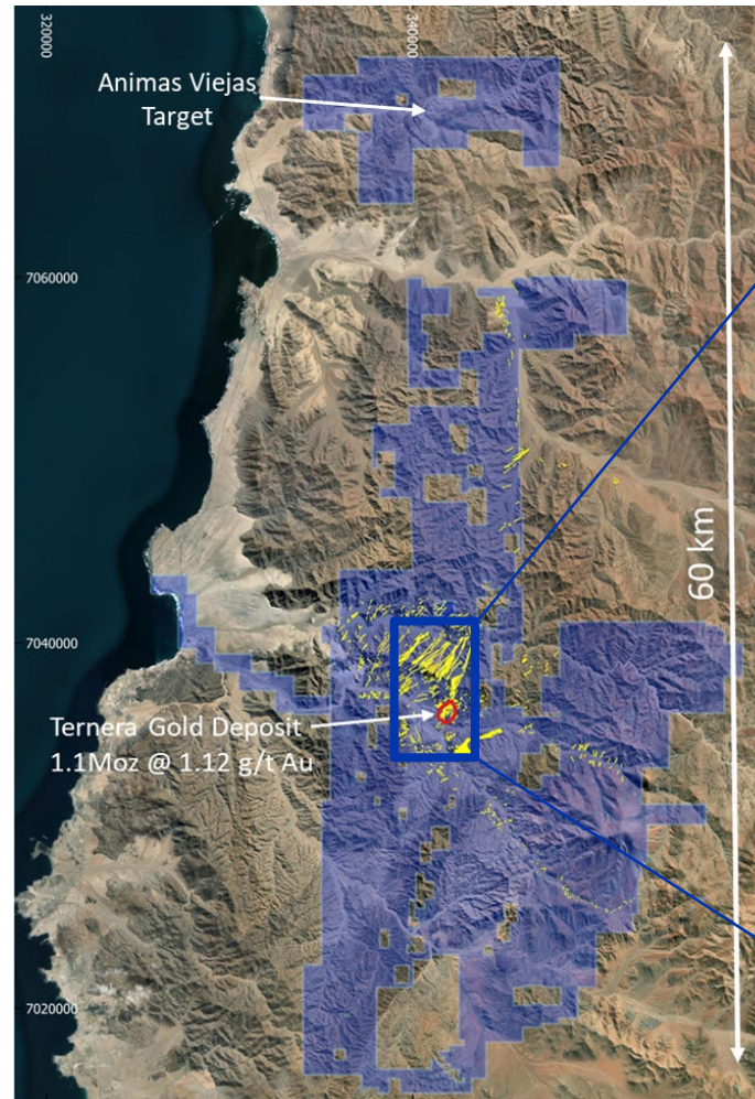
El Zorro Gold Project concession map. Yellow indicates mapped intrusions (EZT) prospective for gold mineralisation
