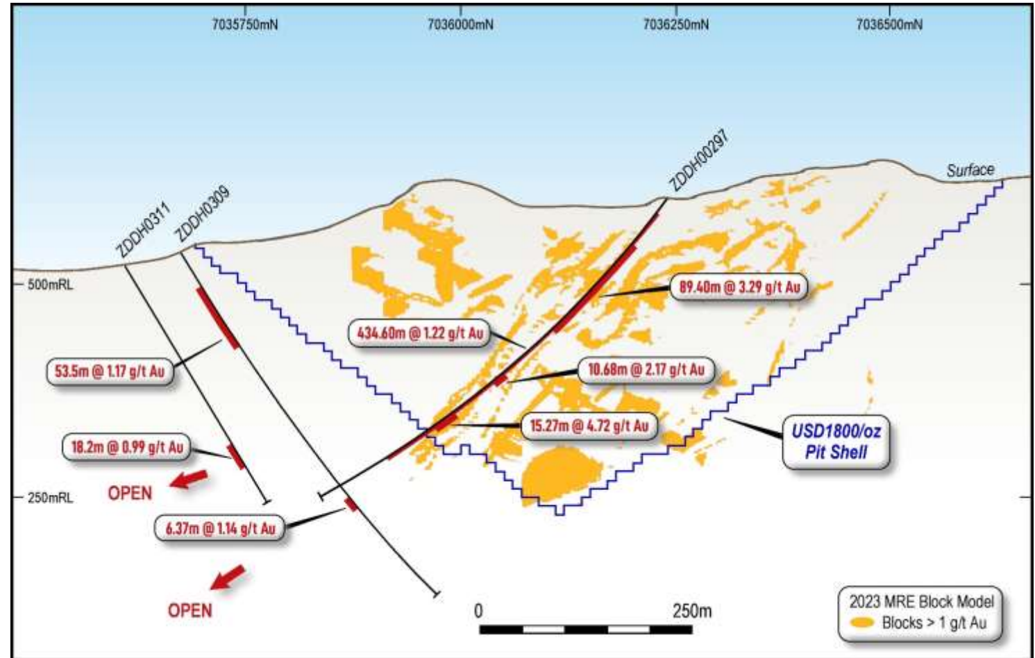
Ternera Gold Deposit Section looking west: Block Model of indicated and inferred resources showing blocks >1.00g/t Au.
