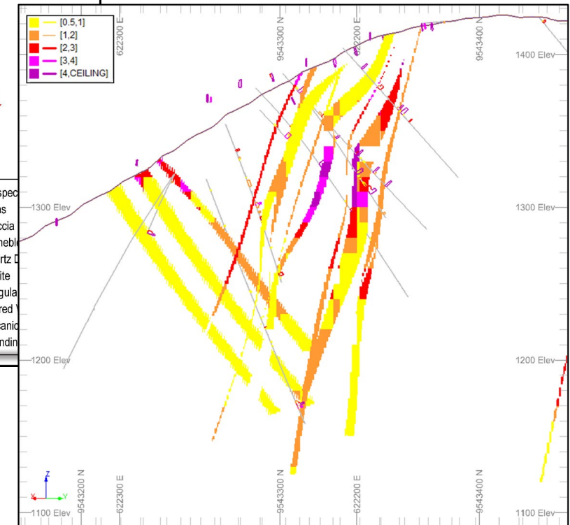
Cross Section looking northeast through Cerro Verde
