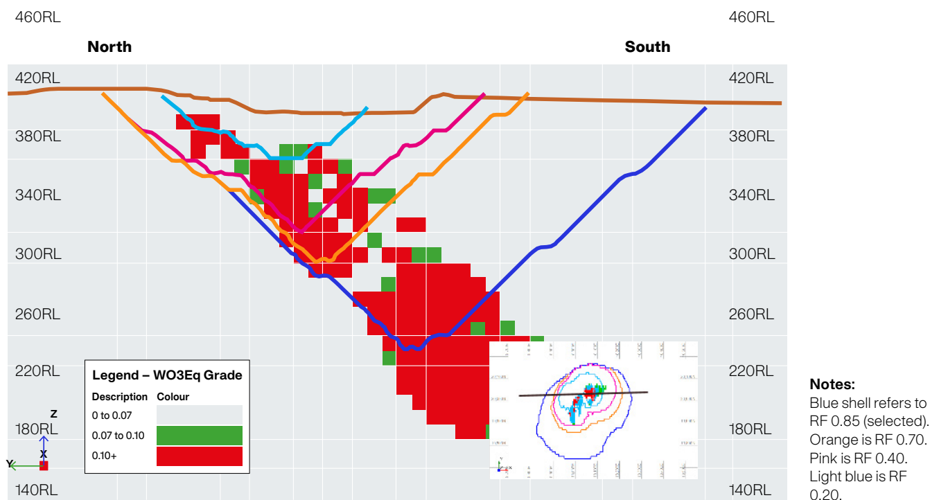
Figure 19: Pit optimisation shells – Cross-section view – North-South
