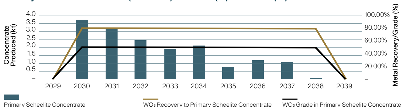
Figure 43: Primary Scheelite Concentrate Produced (kt) and Grade (%)
