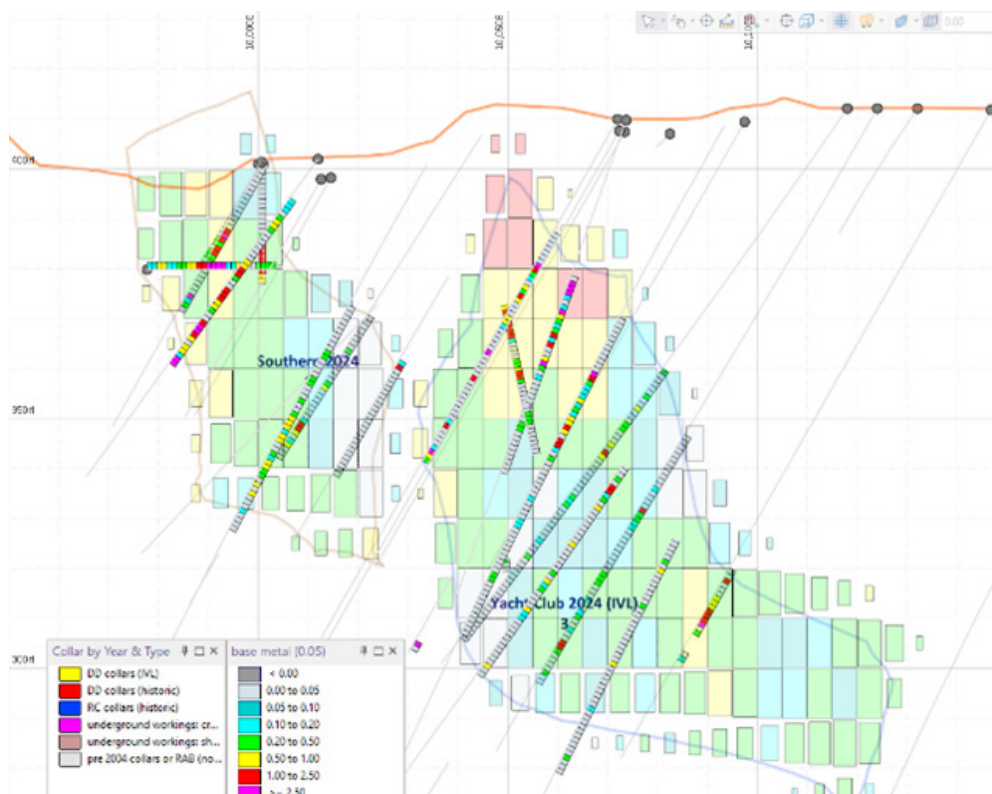
Figure 15: Cross Section 20,030mN – Block Model and Drill Holes for WO 3
