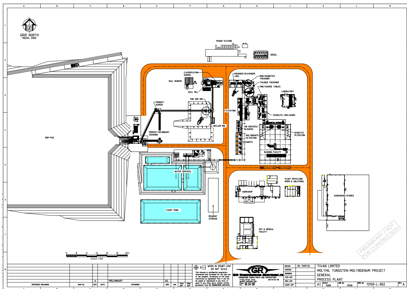
Figure 26: Process Plant Layout showing locations of key areas of the Molyhil Tungsten Project
