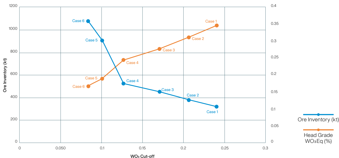
Figure 23: Preliminary Underground Inventory (grade-tonnage curve) below the RF 0.85 open pit
