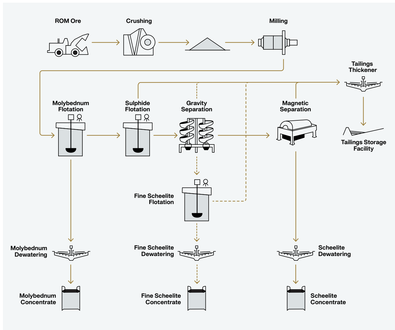
Figure 25: Molyhil Tungsten Project Process Flowsheet
