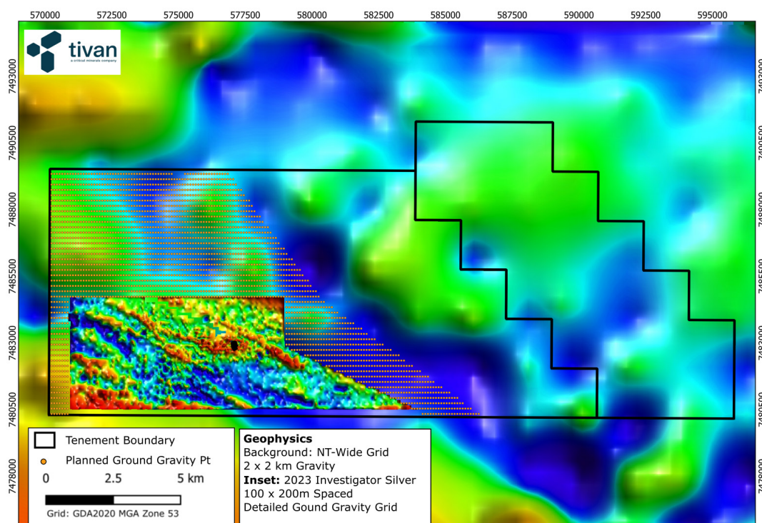
Figure 13: NT-wide 2 km × 2 km gravity grid with detailed survey overlay, tenements, and planned stations
