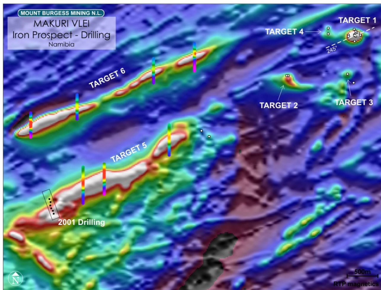
Aeromagnetics - Makuri Vlei Targets
