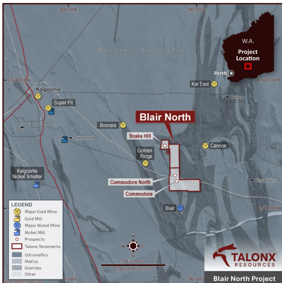
Figure 2. Blair North Project map showing key gold prospects
