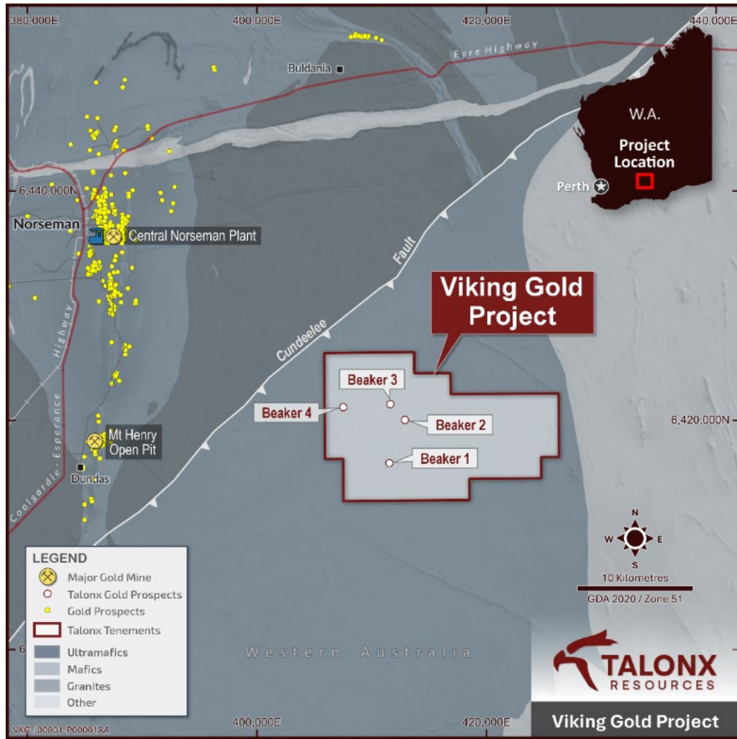
Figure 3. Viking Gold Project location
