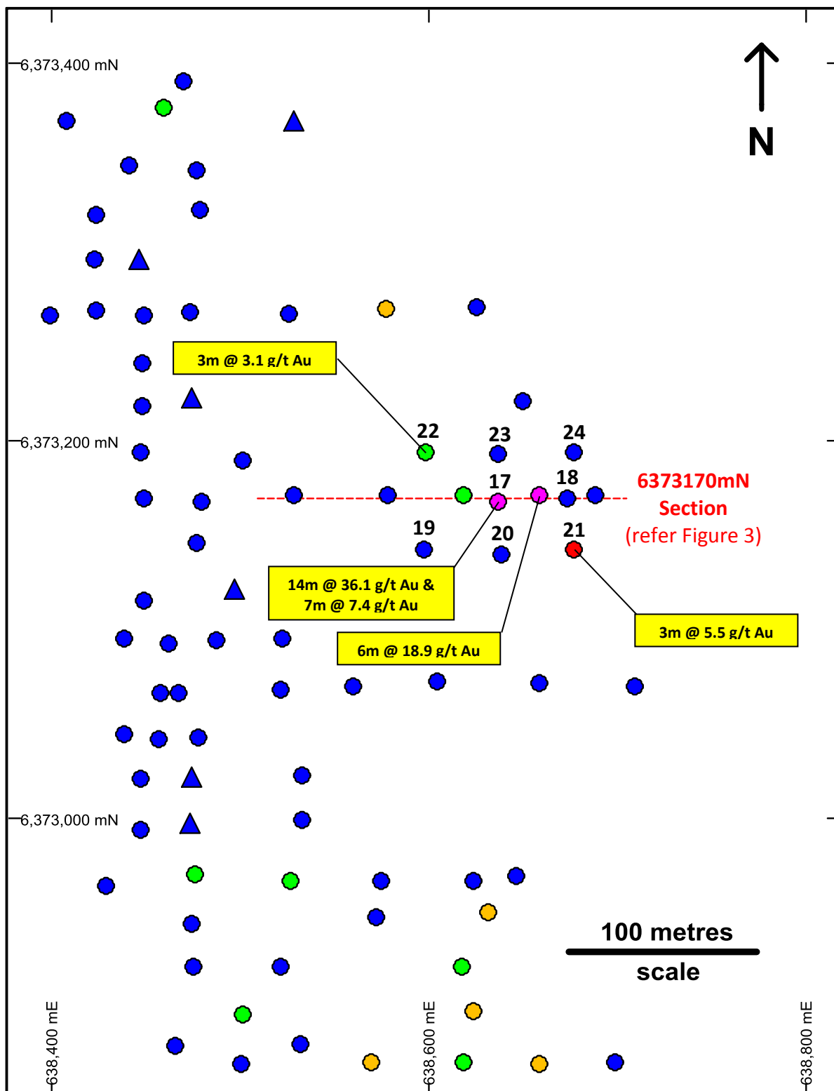
Figure 2. Target 3: Location of recent drilling on maximum gold in hole collar plan (insert to Figure 1)
