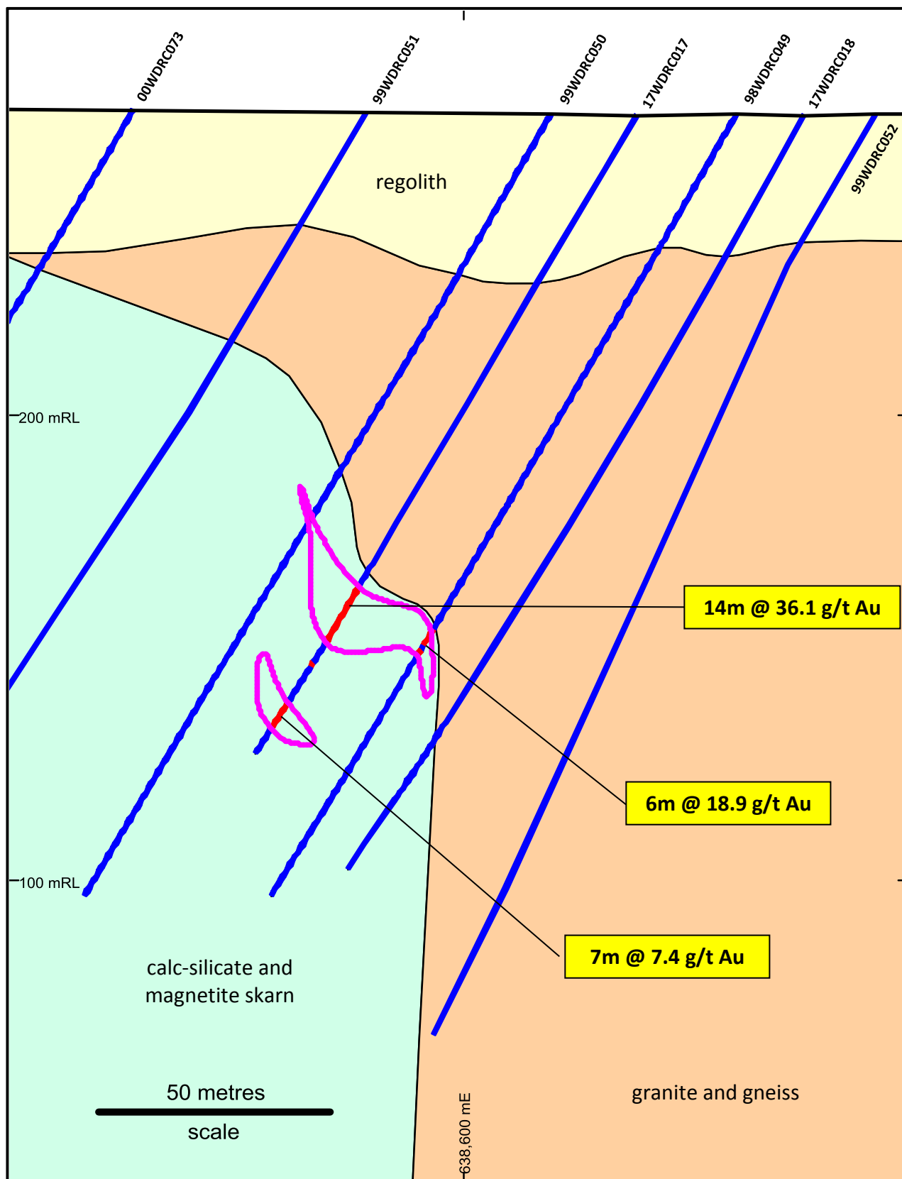
Figure 3. Target 3: 6373170mN Cross-Section with gold drilling results
