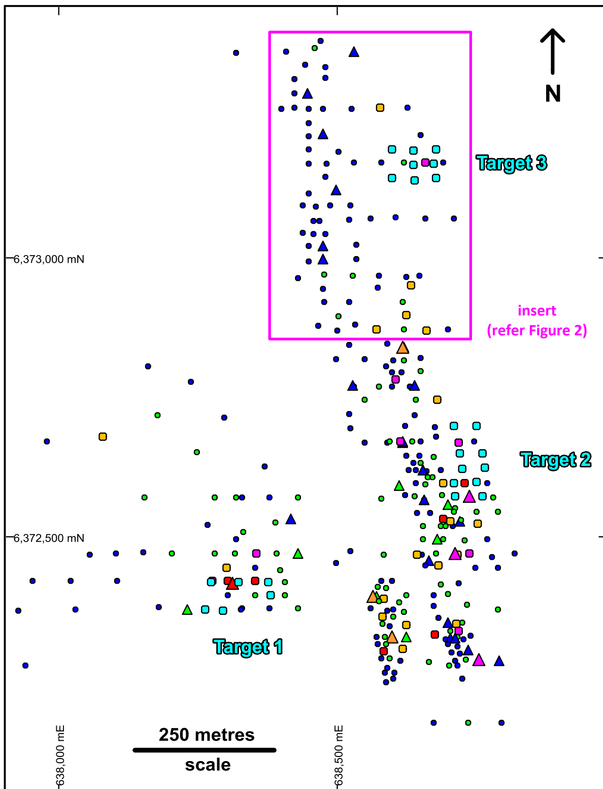
Figure 1. Weednanna: Location of recent drilling on maximum gold in hole collar plan
