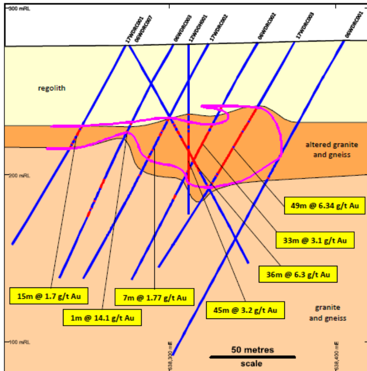
Target 1: Cross section with gold drilling results
