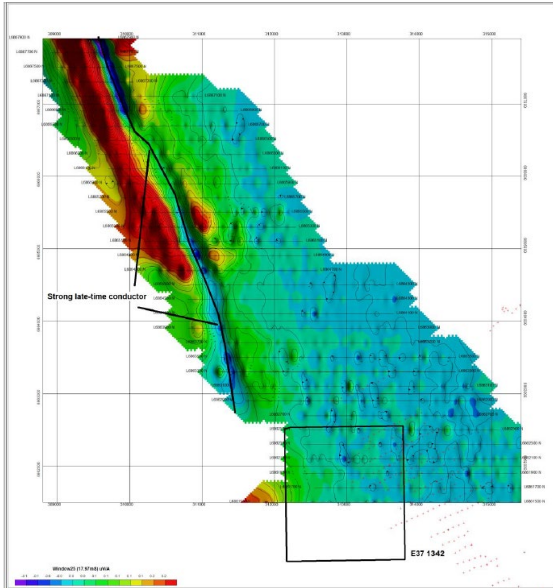
FIGURE 4: WILSON MOVING LOOP TDEM SURVEY. COLOUR SHADED RELIEF IMAGE OF DB/DT RESPONSE, VERTICAL (Z) COMPONENT, DECAY WINDOW 25 (17.968MILLISECONDS), WITH AN OUTLINE OF E37/1342 AND SURVEY LINES.
