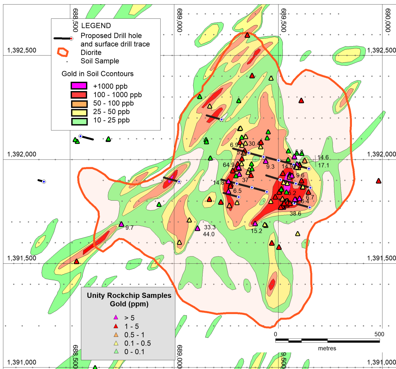
Figure 2: Gold in soil anomalies, rock chip sample gold results & proposed drill holes at Ngot Central Prospect on the interpreted outline of the diorite intrusion (orange outline & shading).
