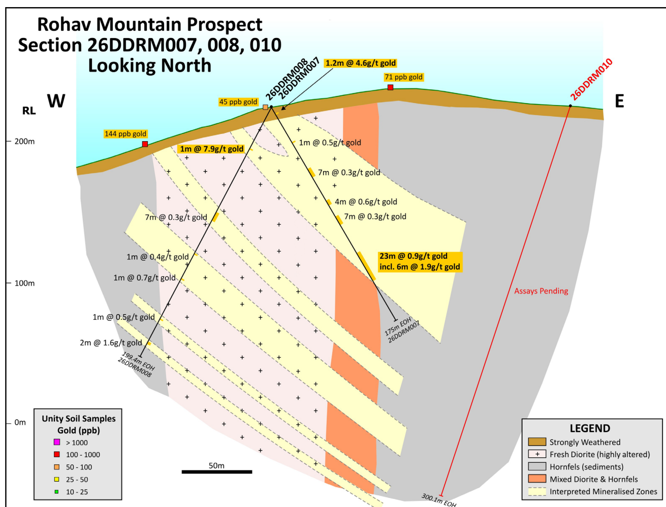
Figure 2: Drill section at the Rohav Mountain Prospect with holes 26DDRM007, 008 & 010.
