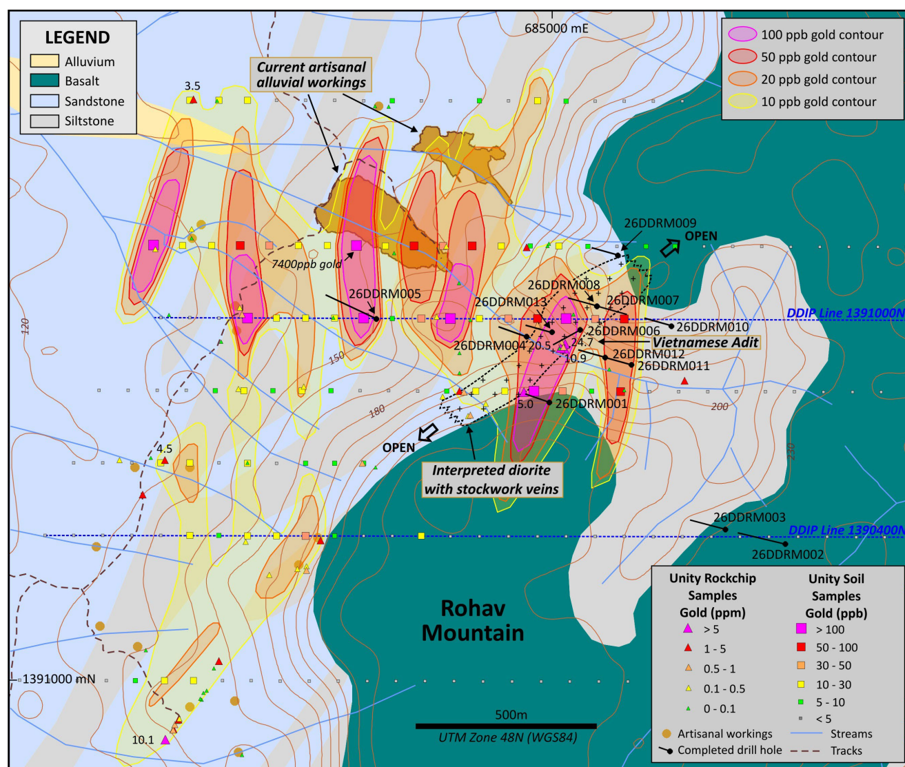
Figure 3: Gold in soil anomalies, rock chip sample gold results, drill holes locations at the Rohav Mountain Prospect on interpreted geology.
