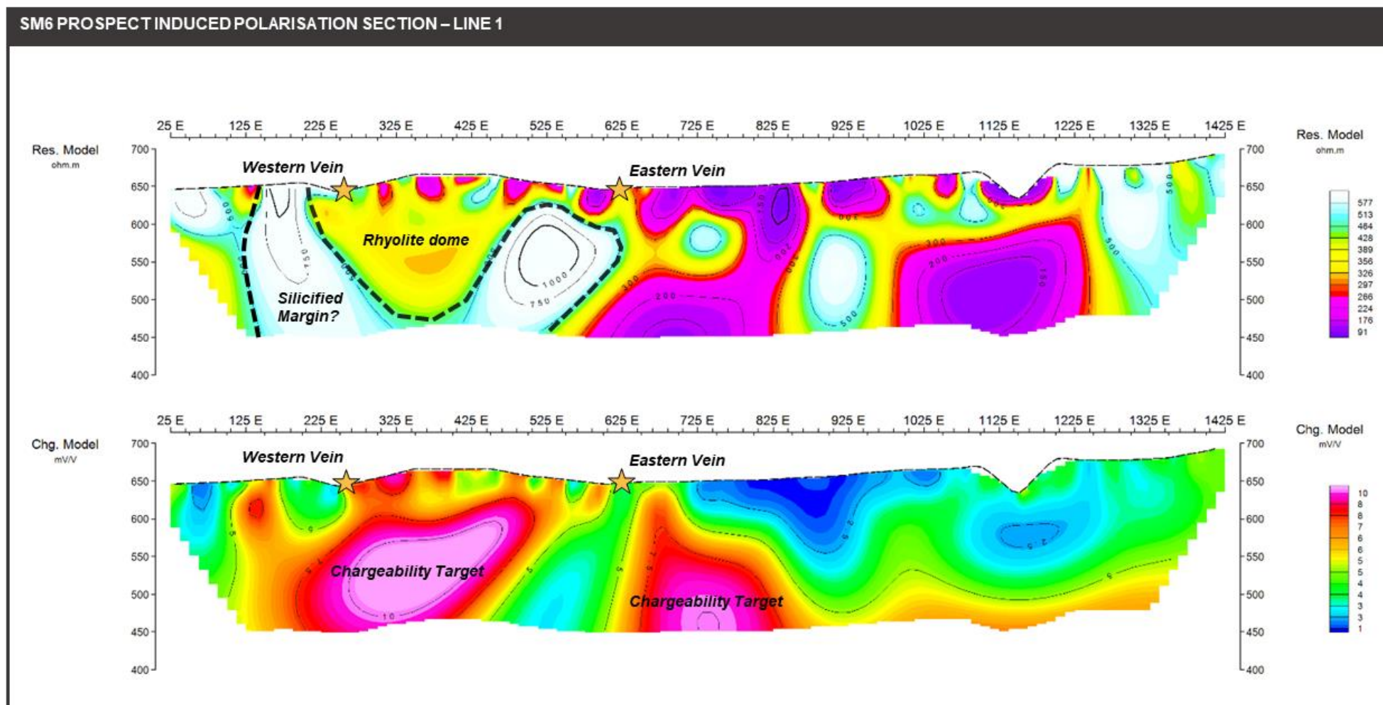
Figure 4: Induced Polarised (IP) inversion showing chargeability targets prospective for rhyolite dome related mineralisation
