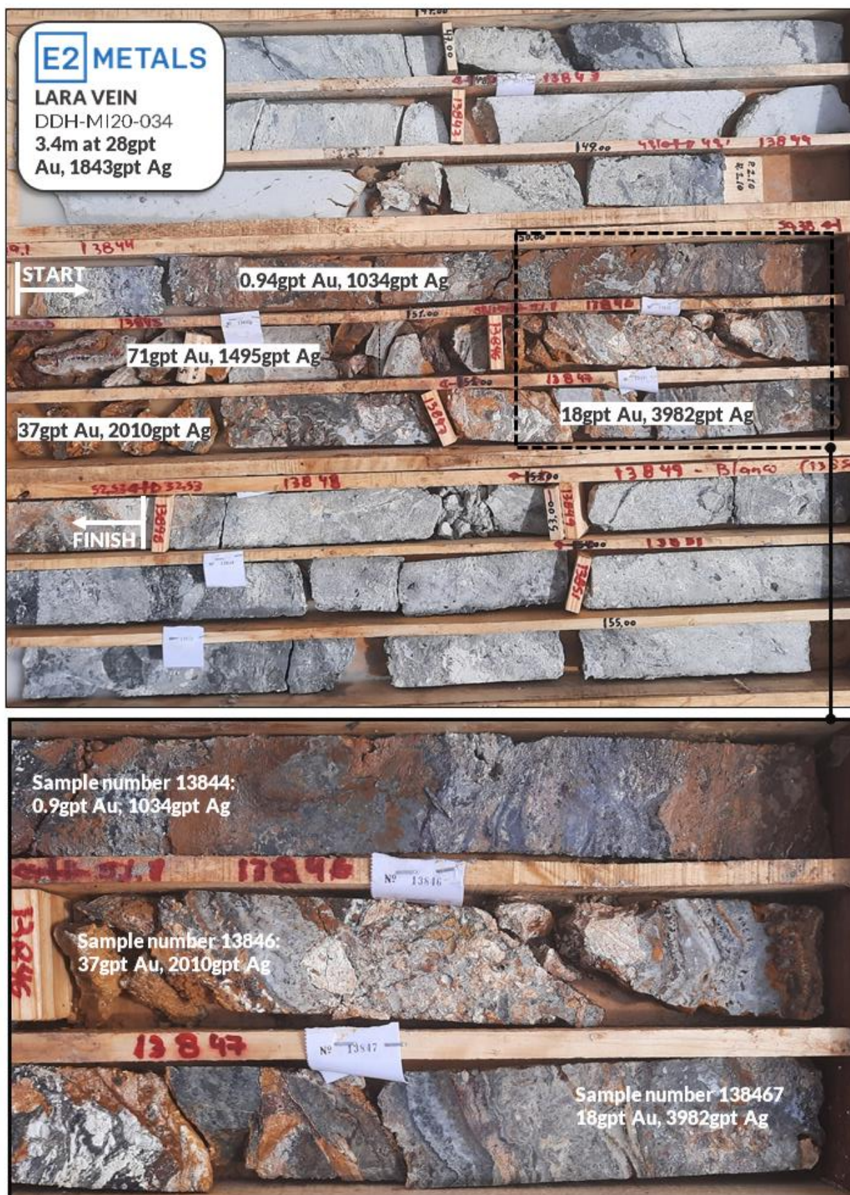
Figure 3: (above) core samples from the Lara Vein and hole DDH-MI20-034 and (below) close up of vein textures
