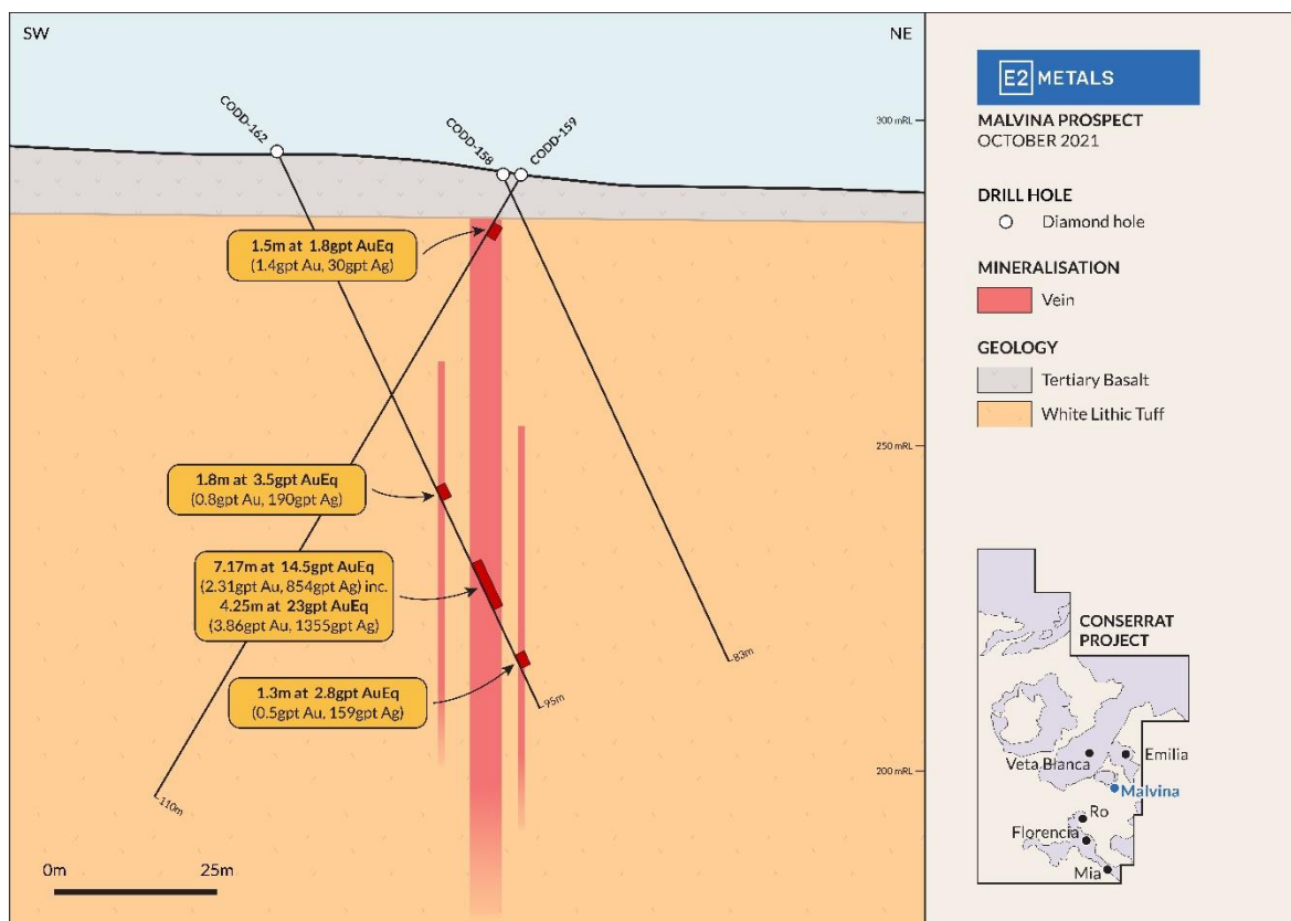
Figure 4: Malvina cross section: hole CODD-162
