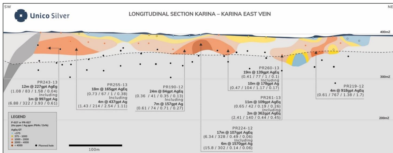
Figure 3: Karina long section
