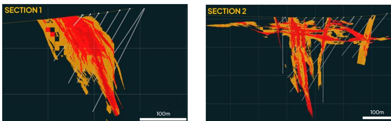
Figure 2: La Negra SE (left) and La Negra(right) block model (AgEq)
