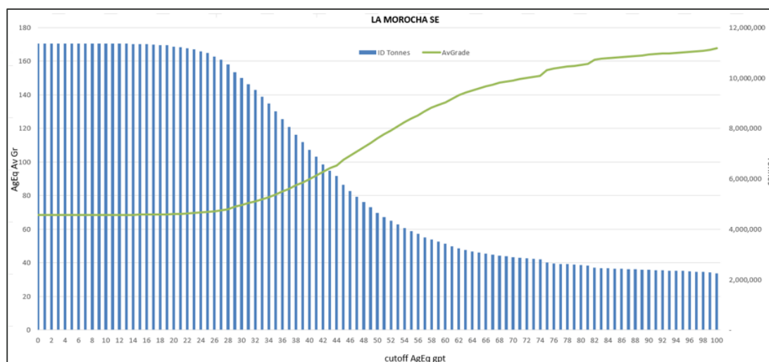
Figure 8-2: La Morocha SE Grade Tonnage Curve
