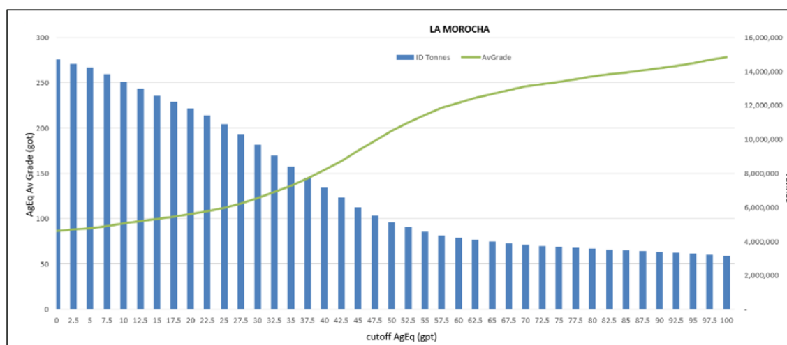
Figure 8-1: La Morocha Grade Tonnage Curve
