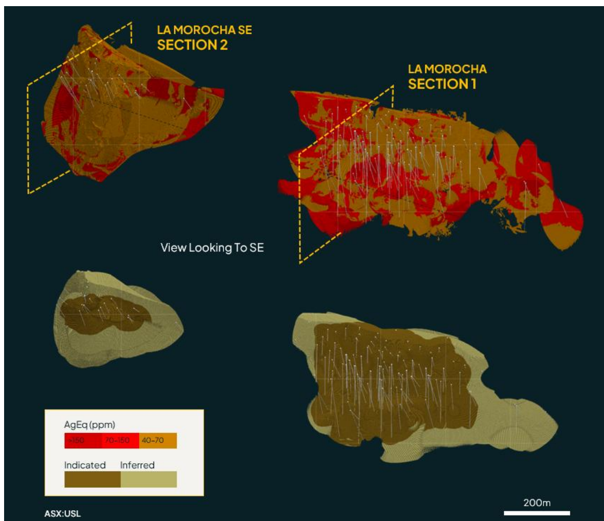
Figure 3: La Morocha – block model (AgEq) and resource category
