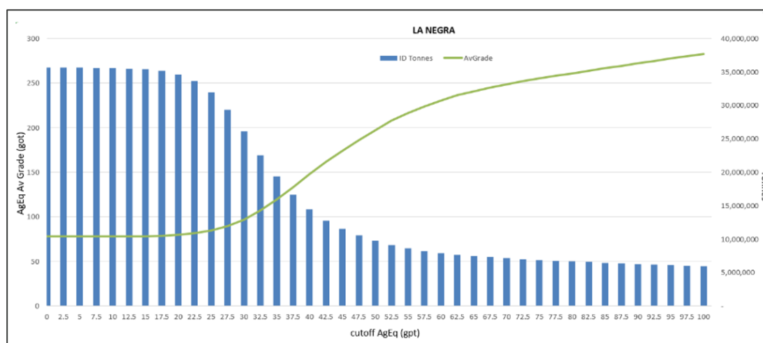
Figure 8-3: La Negra Grade Tonnage Curve
