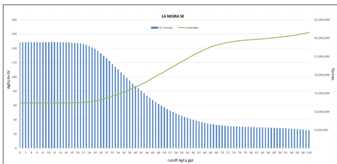
Figure 8-4: La Negra SE Grade Tonnage Curve
