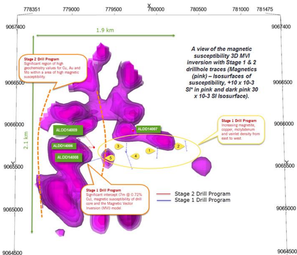
Figure 2 - Alumbre Project magnetic susceptibility 3D MVI model with completed Stage 1 and 2 drillhole program. Detailed logging, sampling and assaying of the Stage 2 drillcore is in progress.
