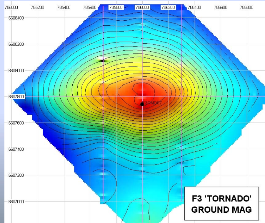
GROUND ANOMALY
