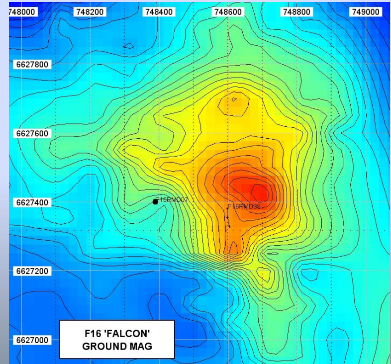
GROUND ANOMALY
