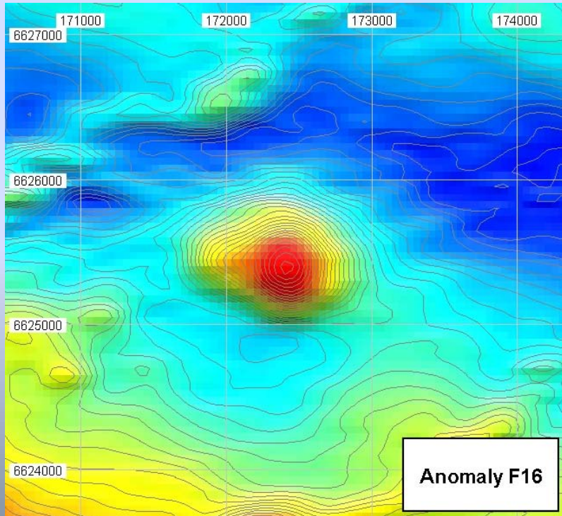
AEROMAGNETIC ANOMALY
