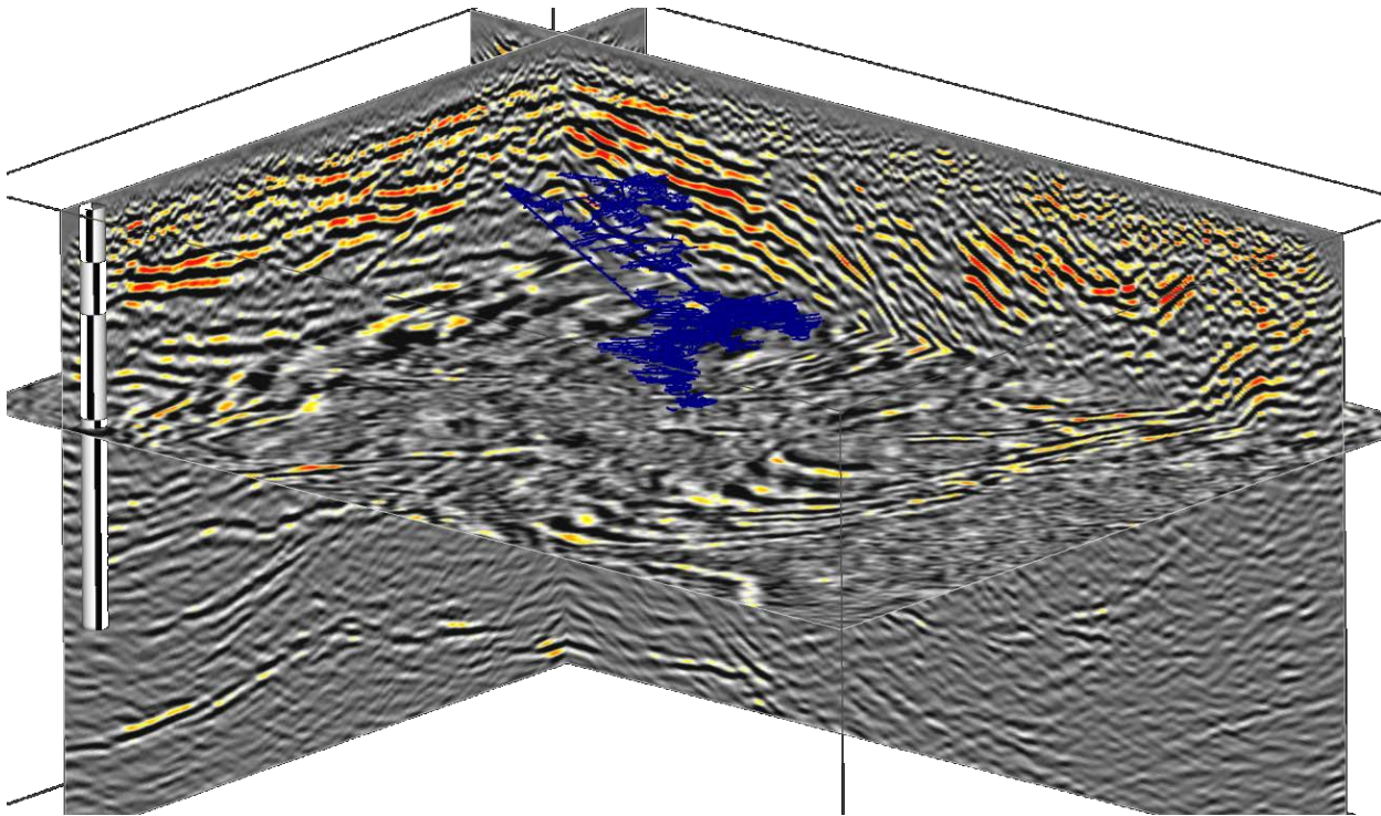
Figure 3: 3D seismic cube showing Darlot mine workings in blue. The brightly coloured areas show strongest reflective zones. Source: DET CRC Annual Conference: Uncovering the Future VII, 12 to 15 September 2017, Hahndorf, South Australia
