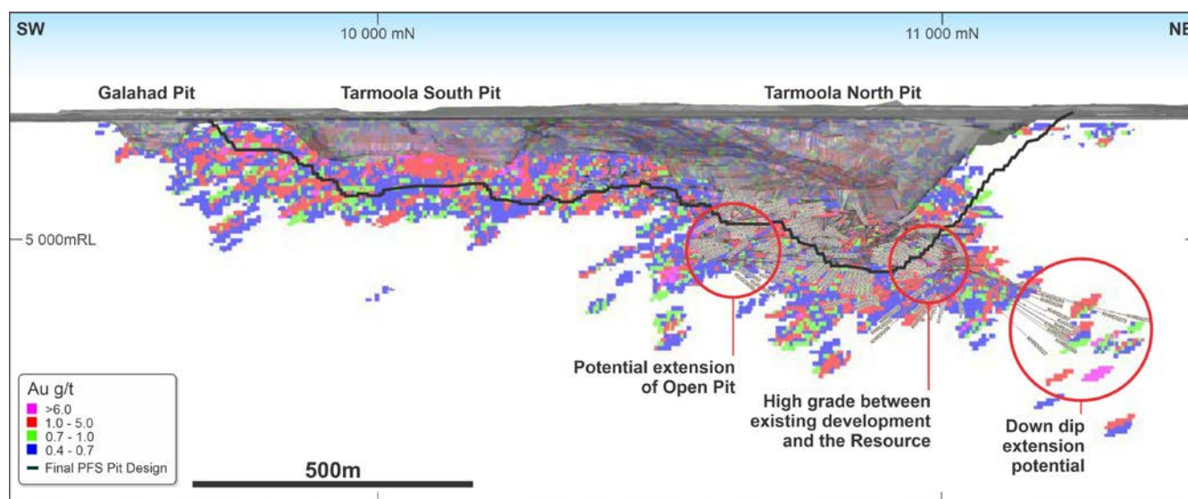
Figure 1: Longitudinal Projection of the KOTH resource model and Tarmoola open pit, looking orthogonal to strike, showing the drill traces of which, the assay results are included in this report.
