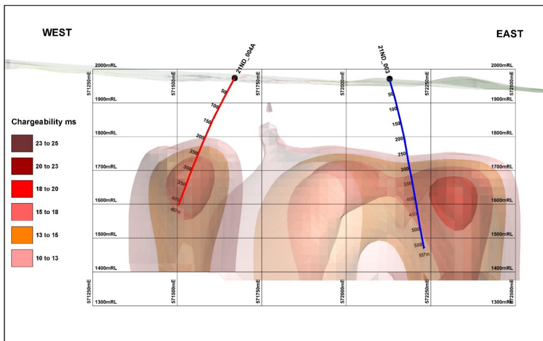
Figure 3. Section looking North with chargeability iso-shells. Drill hole 21ND_003 in blue and just completed drill hole 21ND_004A in red.
