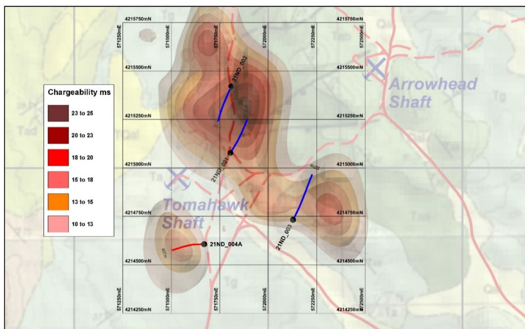
Figure 2. Chargeability anomaly showing actual drill-holes 1, 2 and 3 in blue, with 4A in red
