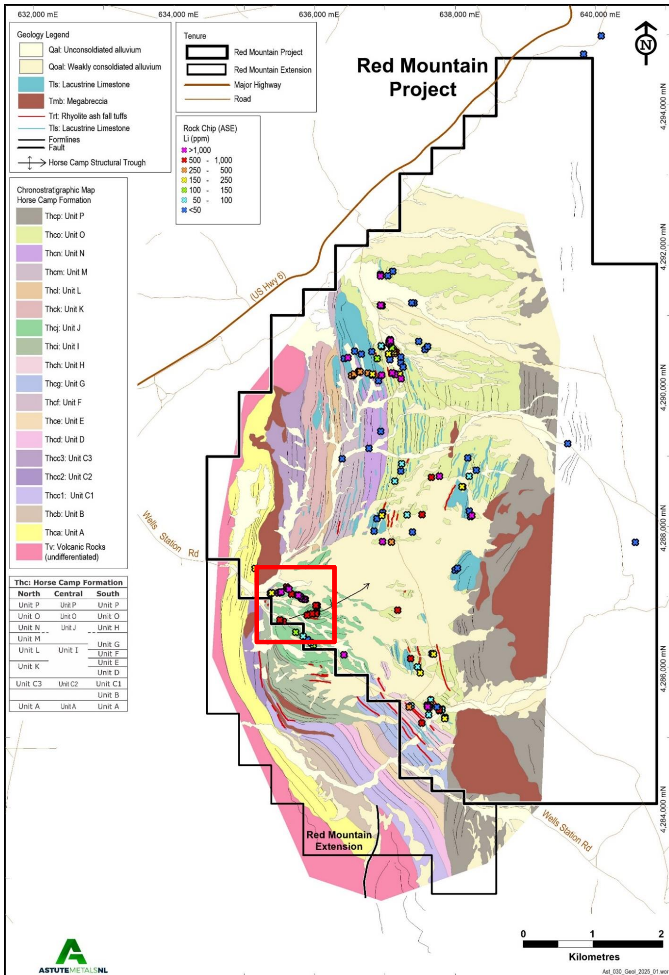
Figure 1. Mapped geology and rock chip lithium geochemistry with red box indicating new lithium zone in Unit J.
