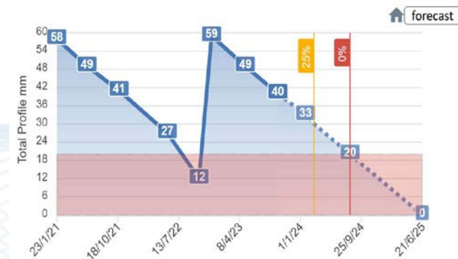
Wear Trend
