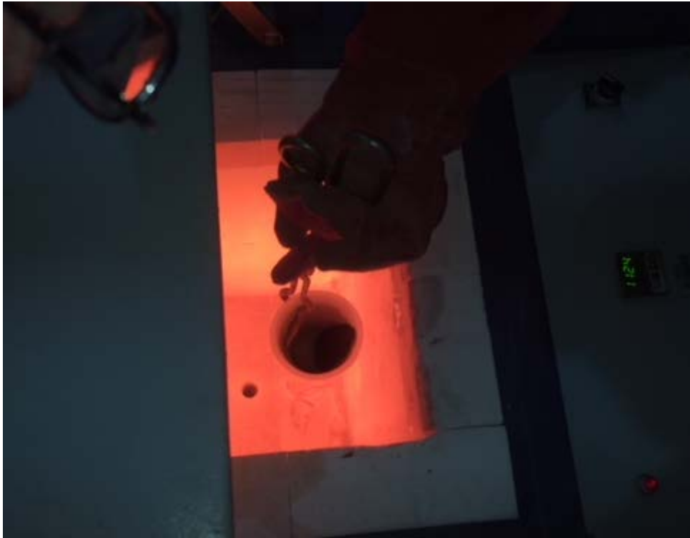
Figure 2. Salt roast testwork underway on samples from the SPD Vanadium Project.
