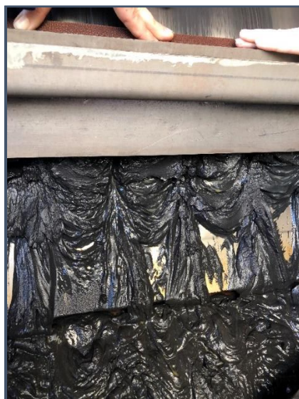
Photo 1 – Concentrate from Low Intensity Magnetic Separator (LIMS)
