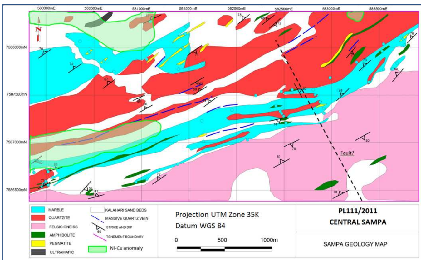
Figure 3 PL111/2011 Solid geology map and coincident Ni-Cu anomalies.
