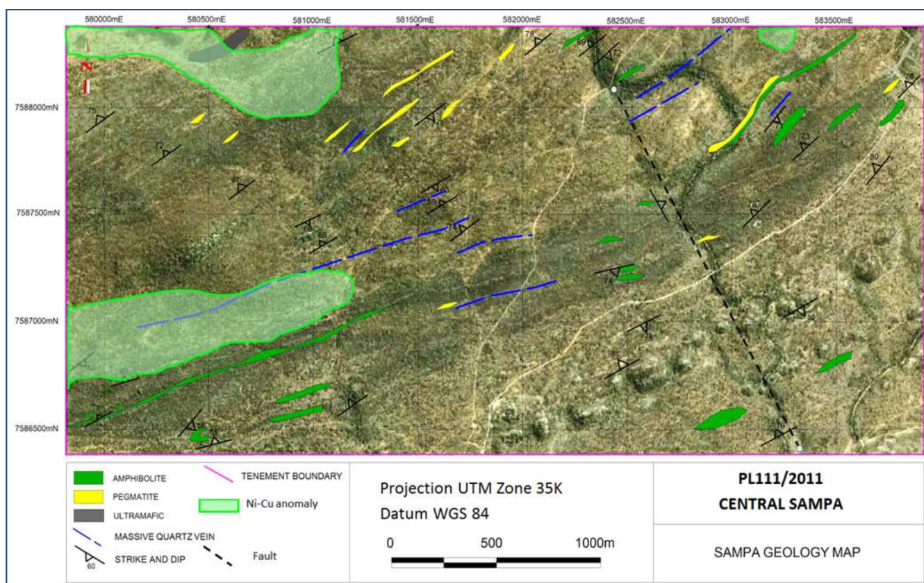
Figure 2 PL111/2011 Satellite image with selected geology and coincident Ni-Cu anomalies.
