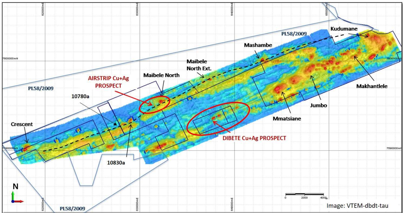
Figure 1: Location of the Airstrip and Dibete Prospects (highlighted in red) within BML's Magogophate exploration portfolio in North-eastern Botswana 8 OF 22 PLANNED HOLES DRILLED.
