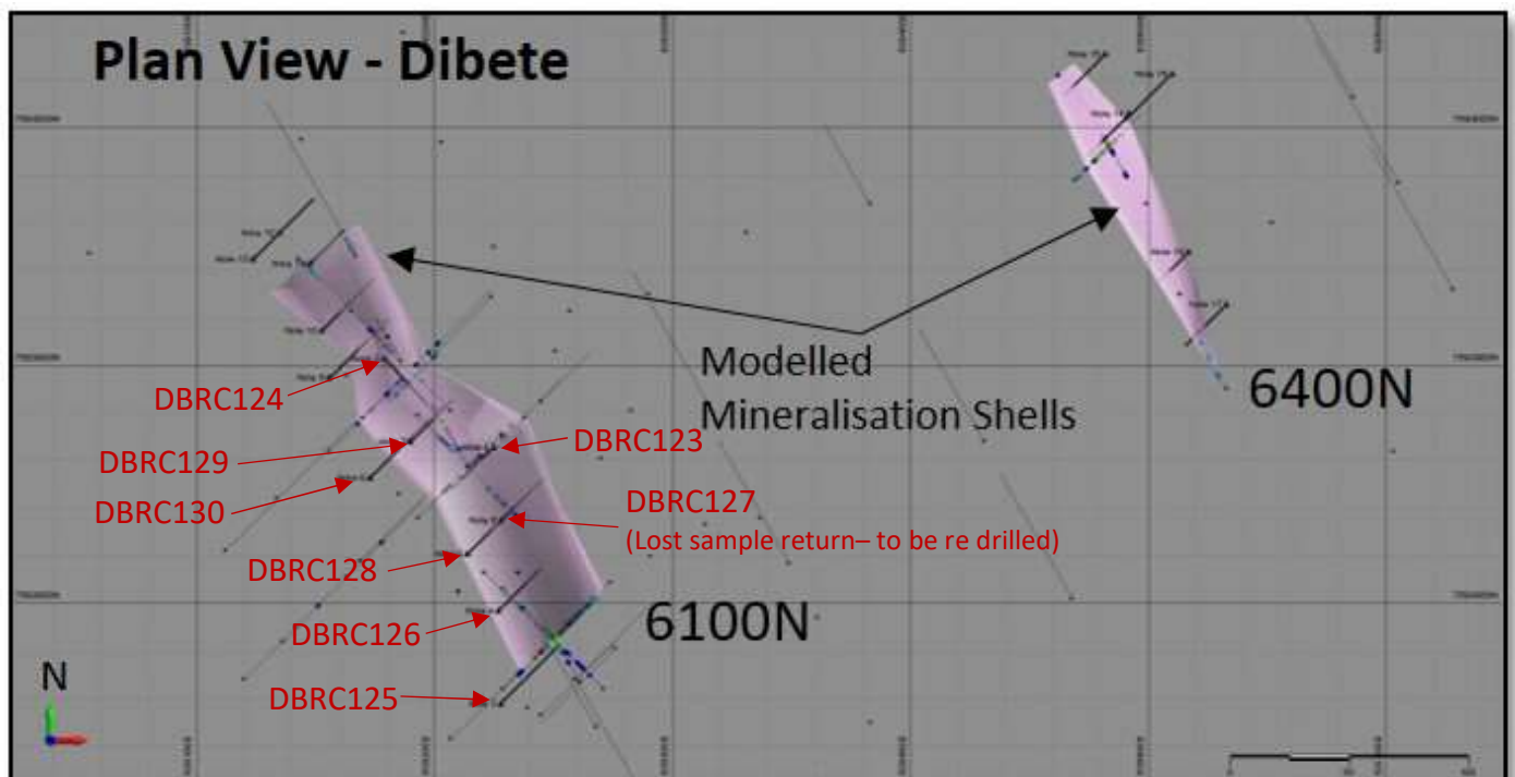
Figure 2: Plan view of the Dibete Project showing modelled mineralisation shells (pink), previous drill holes (thin grey traces) and proposed holes (thicker black traces). Holes completed to date are indicated by red text and arrows.
