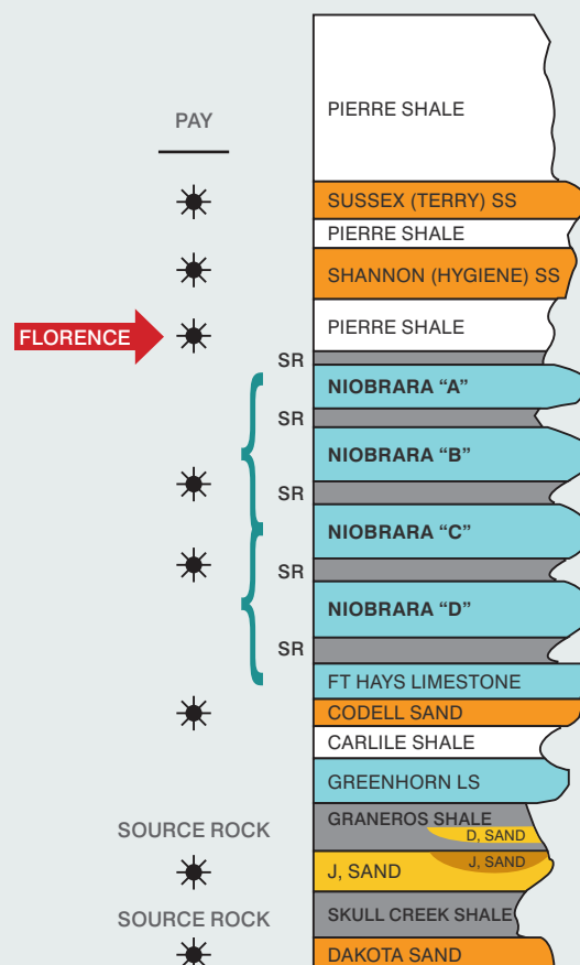
Figure 3. Stratigraphic column, Florence Oilfield.
