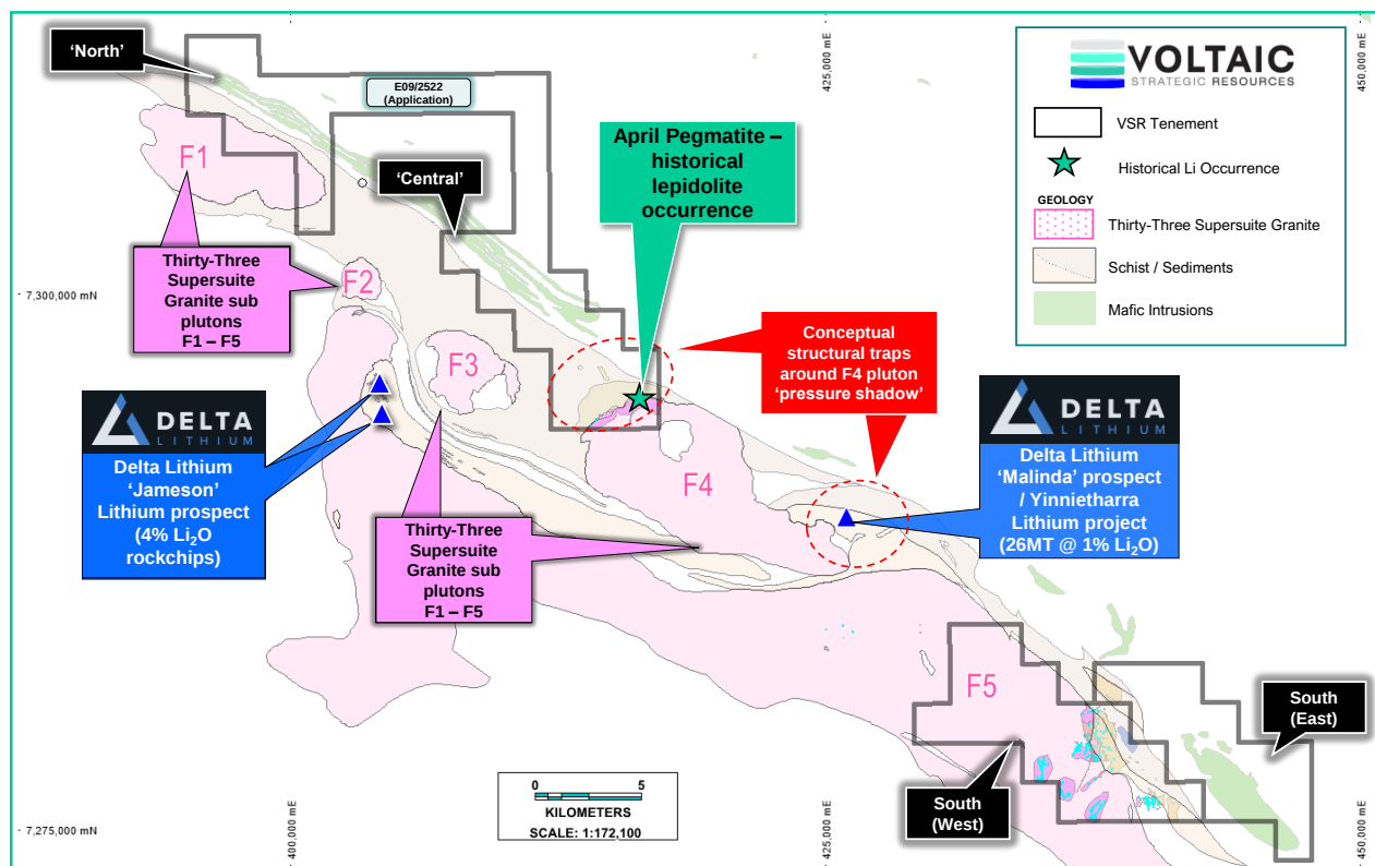
Figure 1. Ti Tree project map. Neighbouring Delta Lithium's Yinnietharra key project areas also shown.
