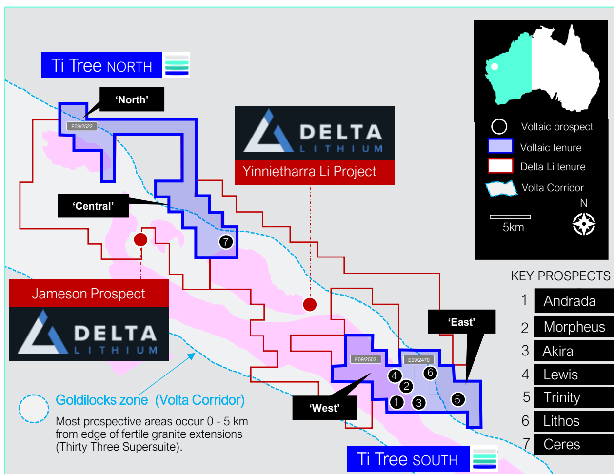
Figure 5. Regional Ti Tree project map with Delta Lithium's Yinnietharra tenure also shown.
