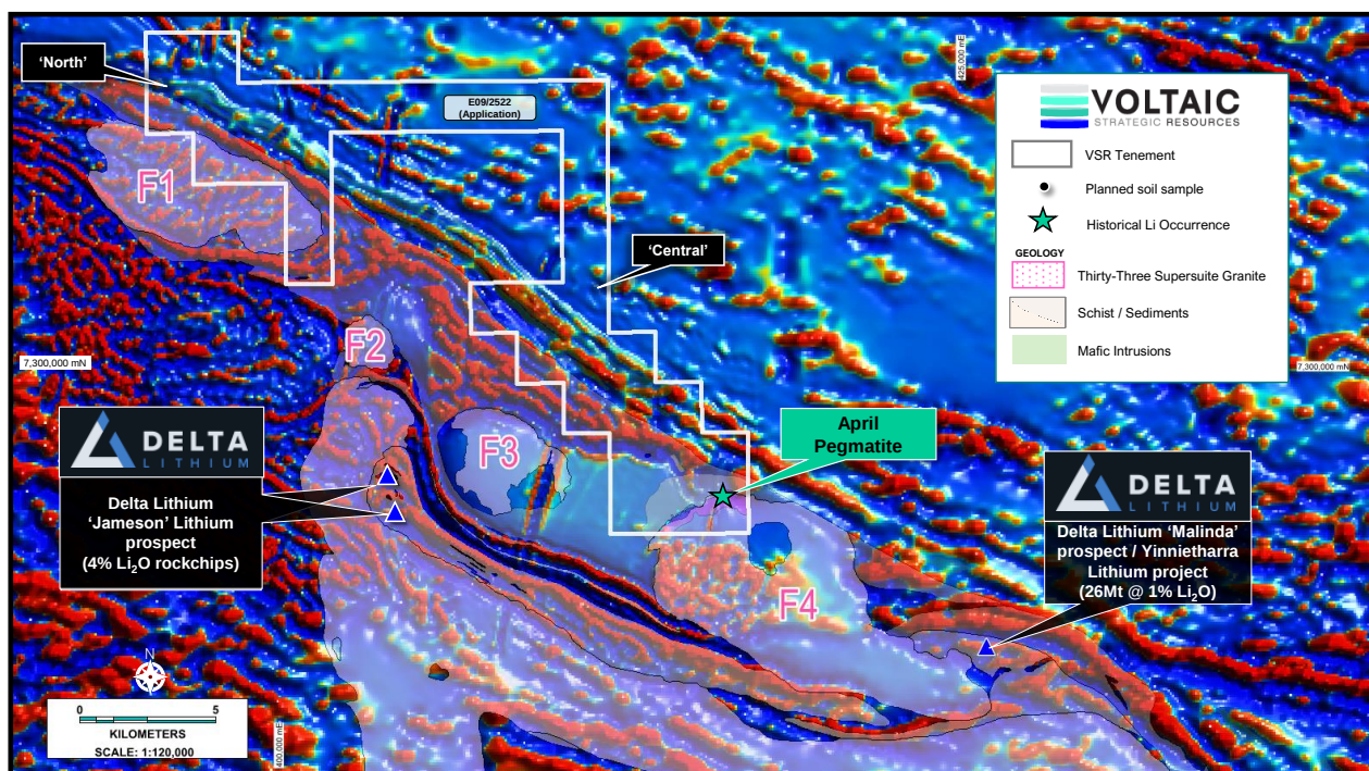
Figure 4. Regional magnetic data (80m, 1VD) across TTN with regional lithium occurrences. Source: GSWA
