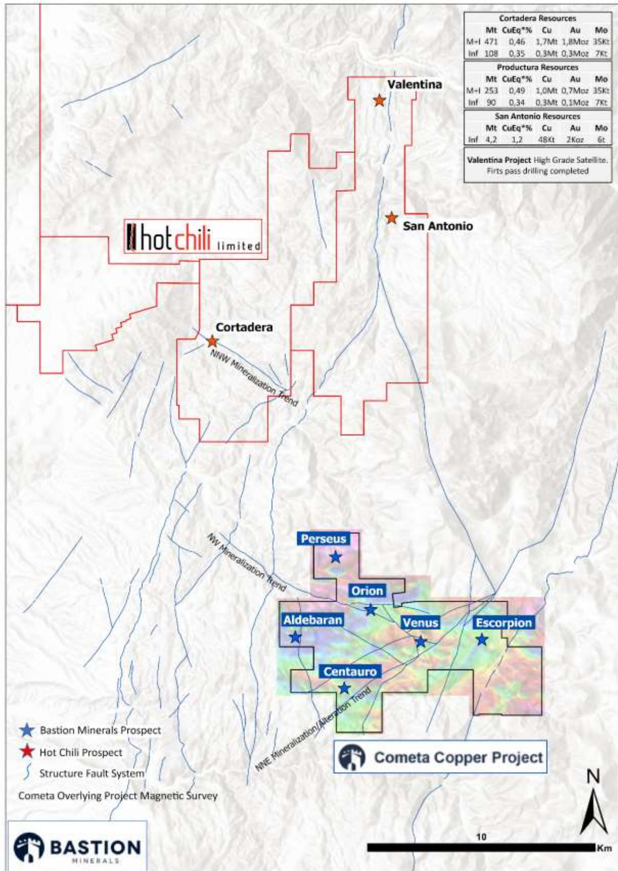
Figure 1: Prospects defined at the Cometa project. Note the northeast trend on which the Venus project is located and the interpreted intersecting NW mineralisation trend. Hot Chili's Productura deposit is west of the map area 8 .
