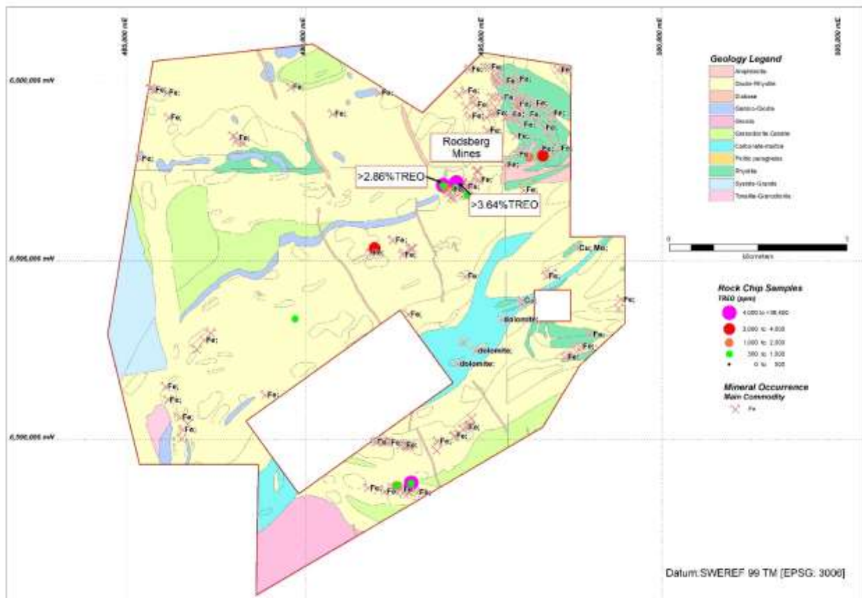
Figure 1: Geology of Bastion ténement showing mineral occurrences and old mines with the major commodity. Samples collected by SGU for rare earth analyses show no systematic sampling has been undertaken.
