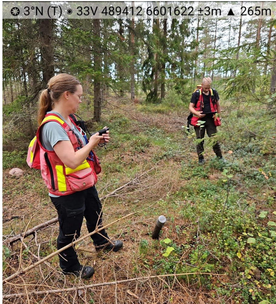
Figure 5: Historical drill hole GGD02 (Grindgruvan 2 in Table 4) in the Striberg property, immediately north of Gyttop. This hole intersected historical copper mineralisation - Bastion has requested access to re-assay this historical drill hole.
