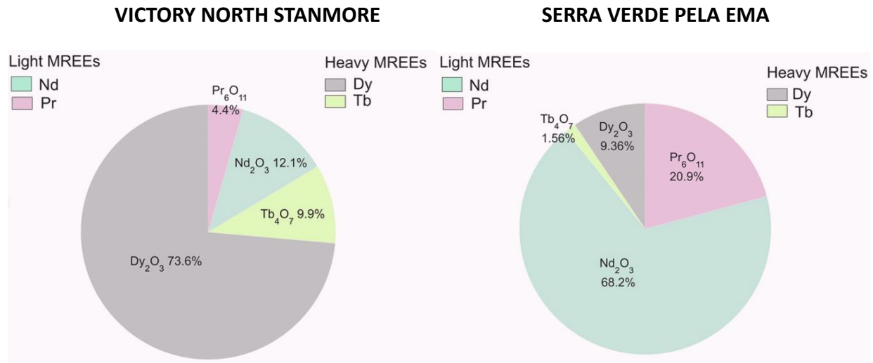
Figure 3: Pie charts comparing relative proportions of the magnet REEs (MREEs), NdPr and DyTb in North Stanmore and Serra Verde Pela Ema Project in Goiás Brazil.
