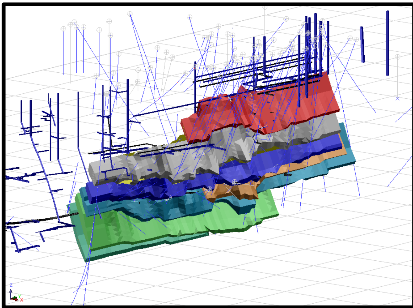
Figure 1 - Oblique view of mineralised domain wireframes
