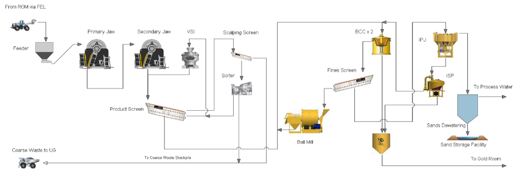
Figure 3 The Hill End Gravity Gold plant with sorter flow sheet. Small and simple.
